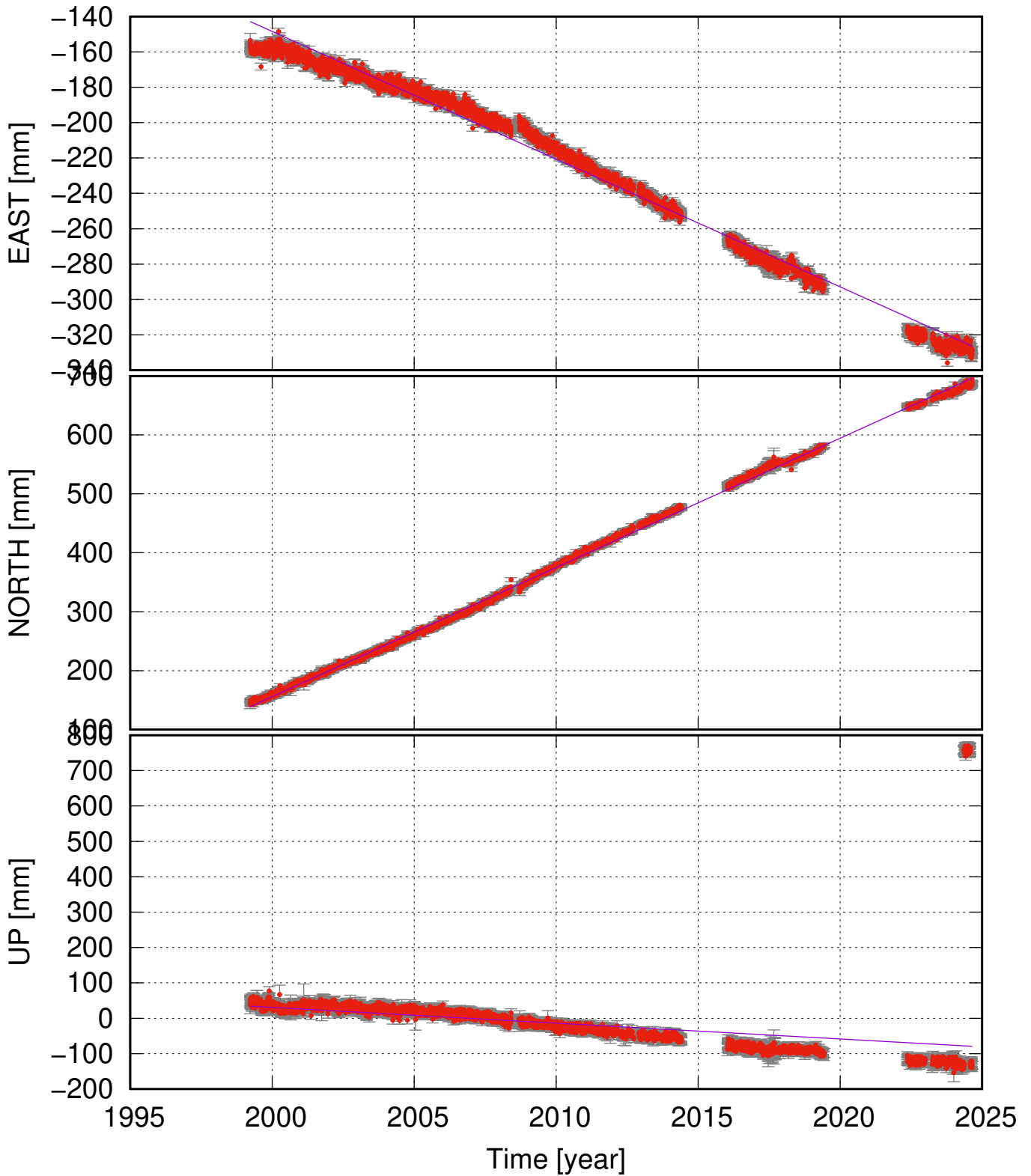
HVER (64.02, -21.18) time series (ITRF 2014) v_e = -7.22 \pm 0.22 ; v_n = 21.93 \pm 0.19 ; v_u = -4.46 \pm 3.67 mm/yr
