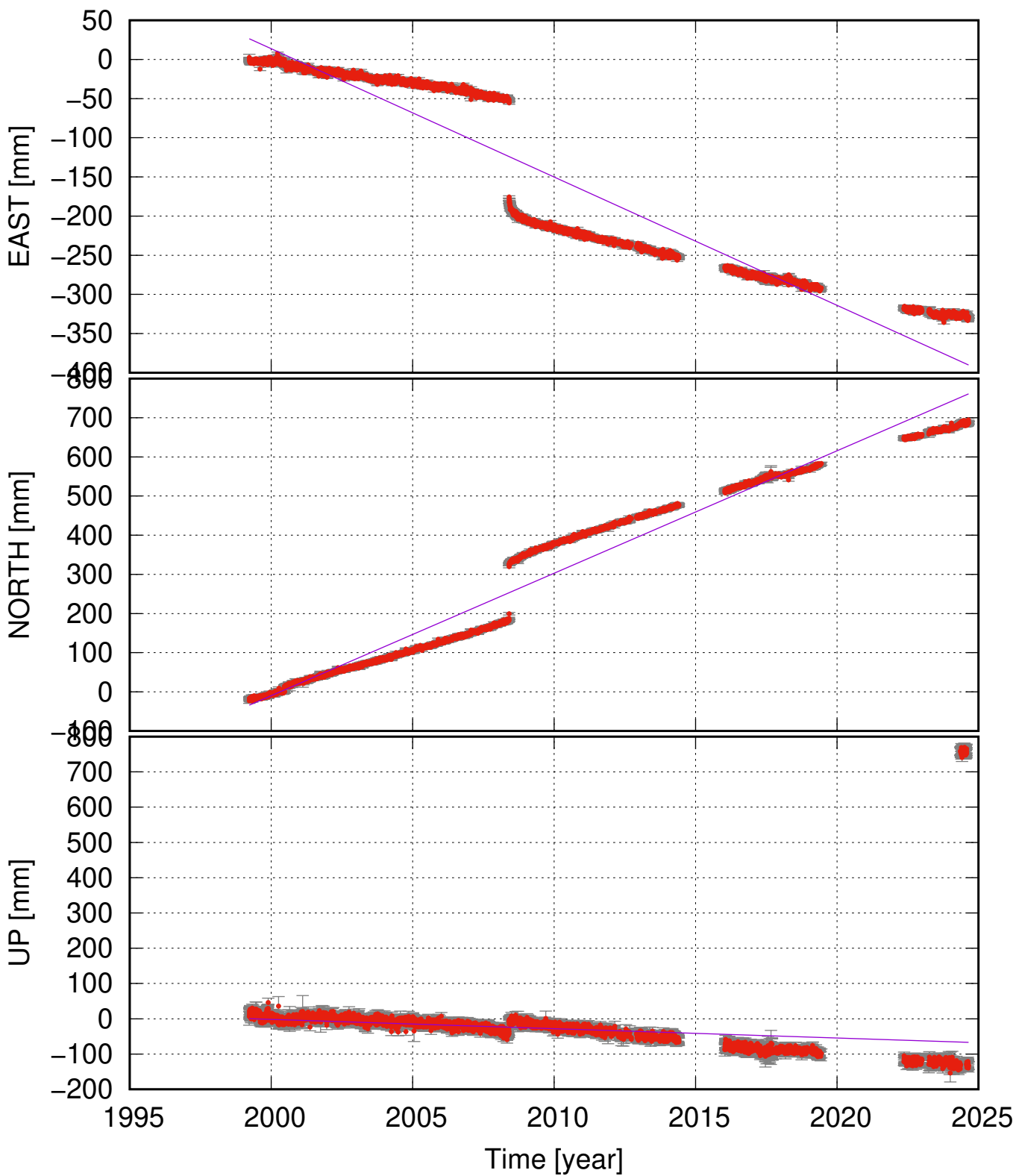
HVER (64.02, -21.18) time series (ITRF 2014) ve = -16.39 ± 1.67; vn = 31.25 ± 1.87; vu = -2.63 ± 3.61 mm/yr
