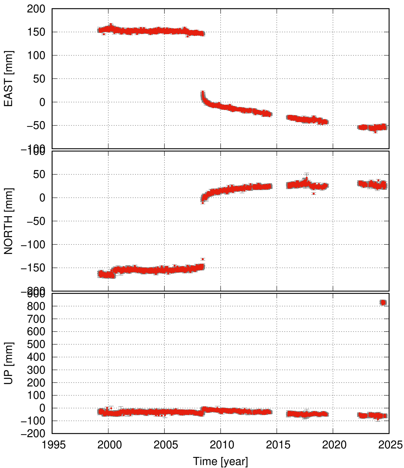
HVER detrended and seasonal signal removed
