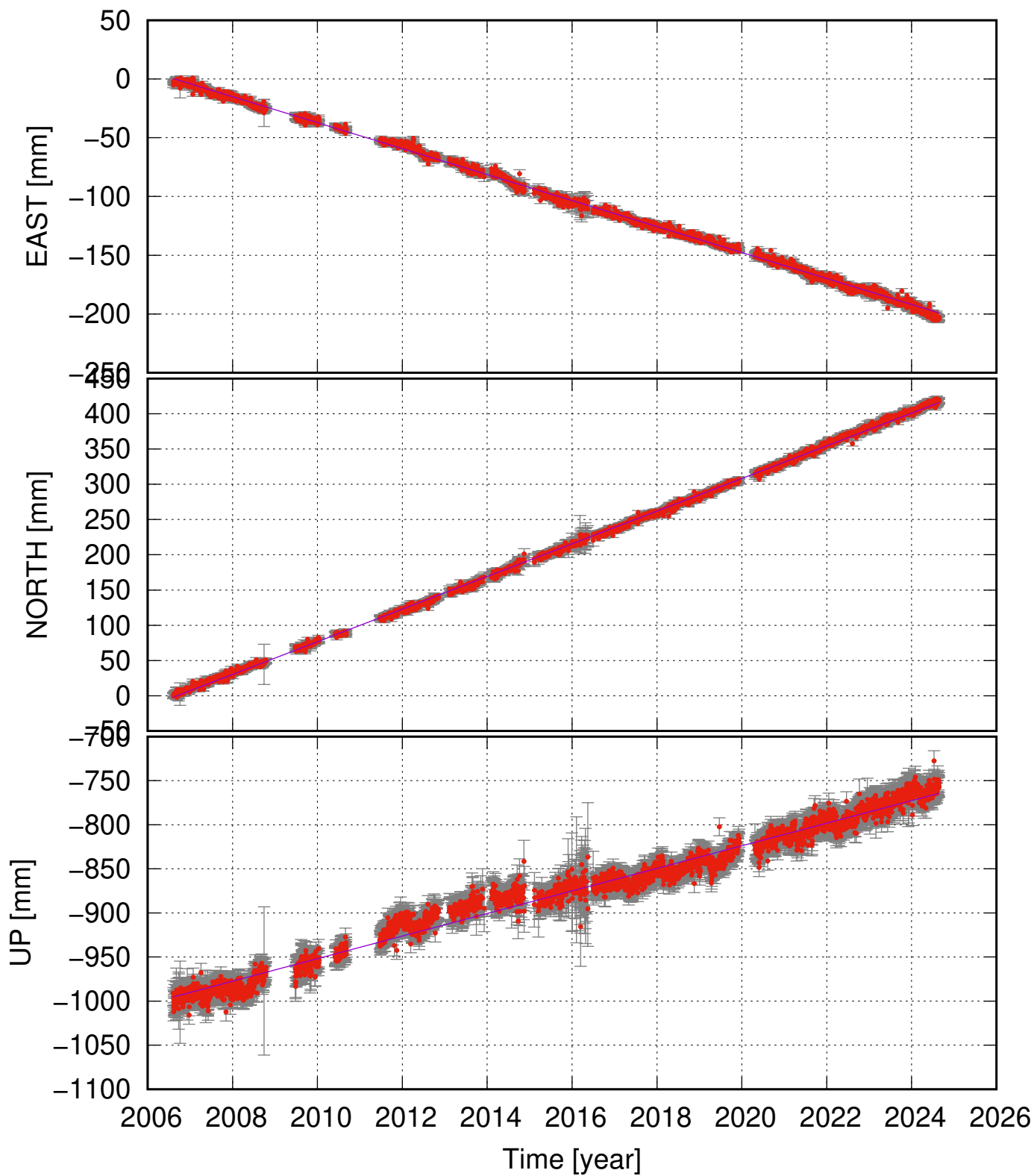
HVEL (64.87, -19.56) time series (ITRF 2014) v_e = -11.05 \pm 0.12 ; v_n = 23.16 \pm 0.16 ; v_u = 12.80 \pm 0.53 mm/yr
