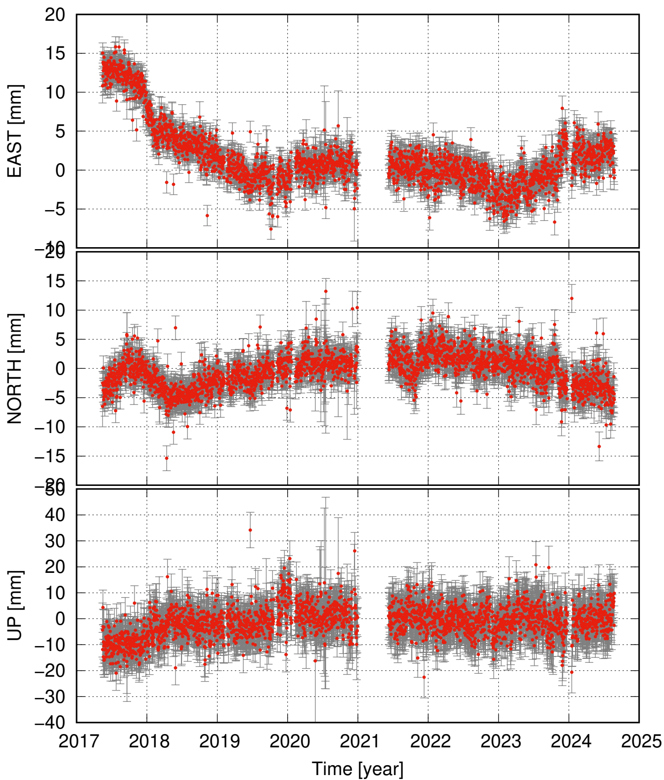
HVEH detrended and seasonal signal removed
