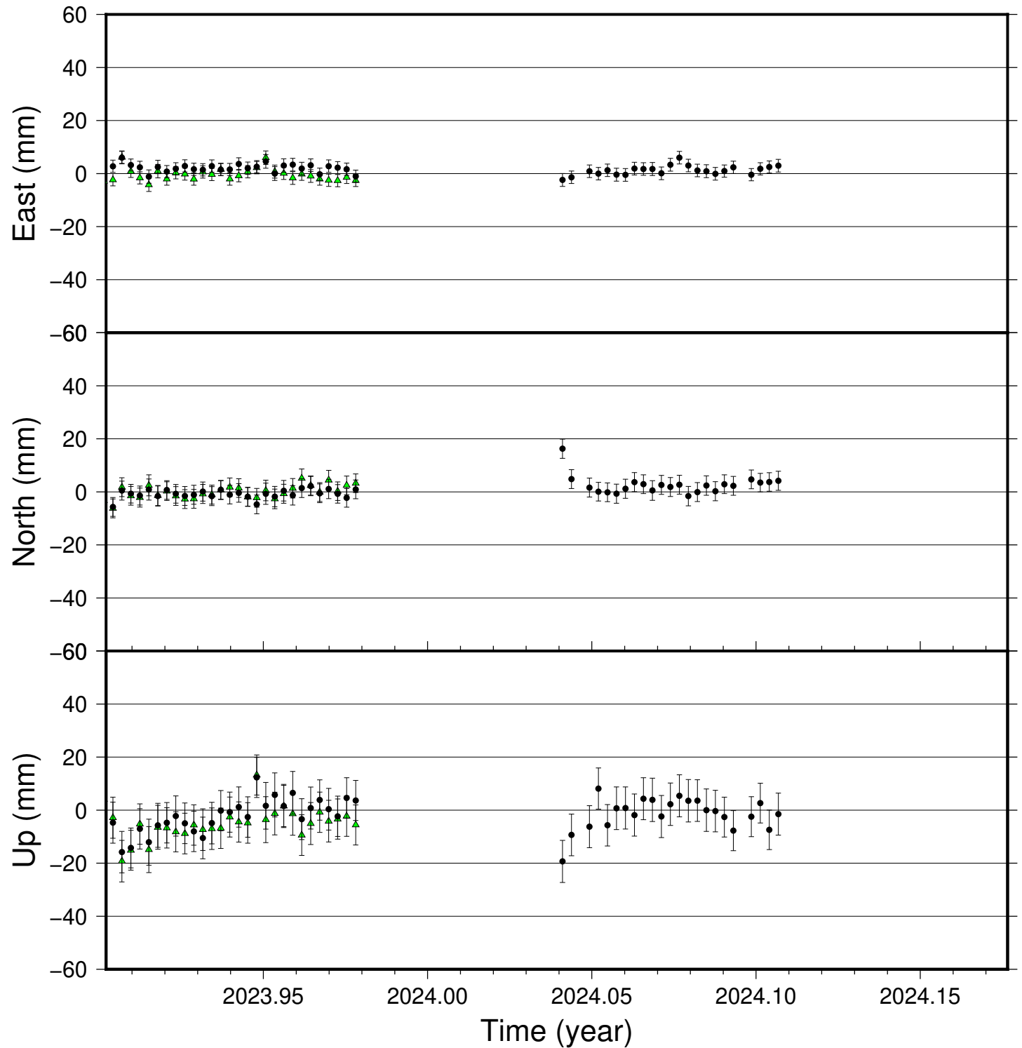
HVEH time series (IGS 2014), last 100 days
