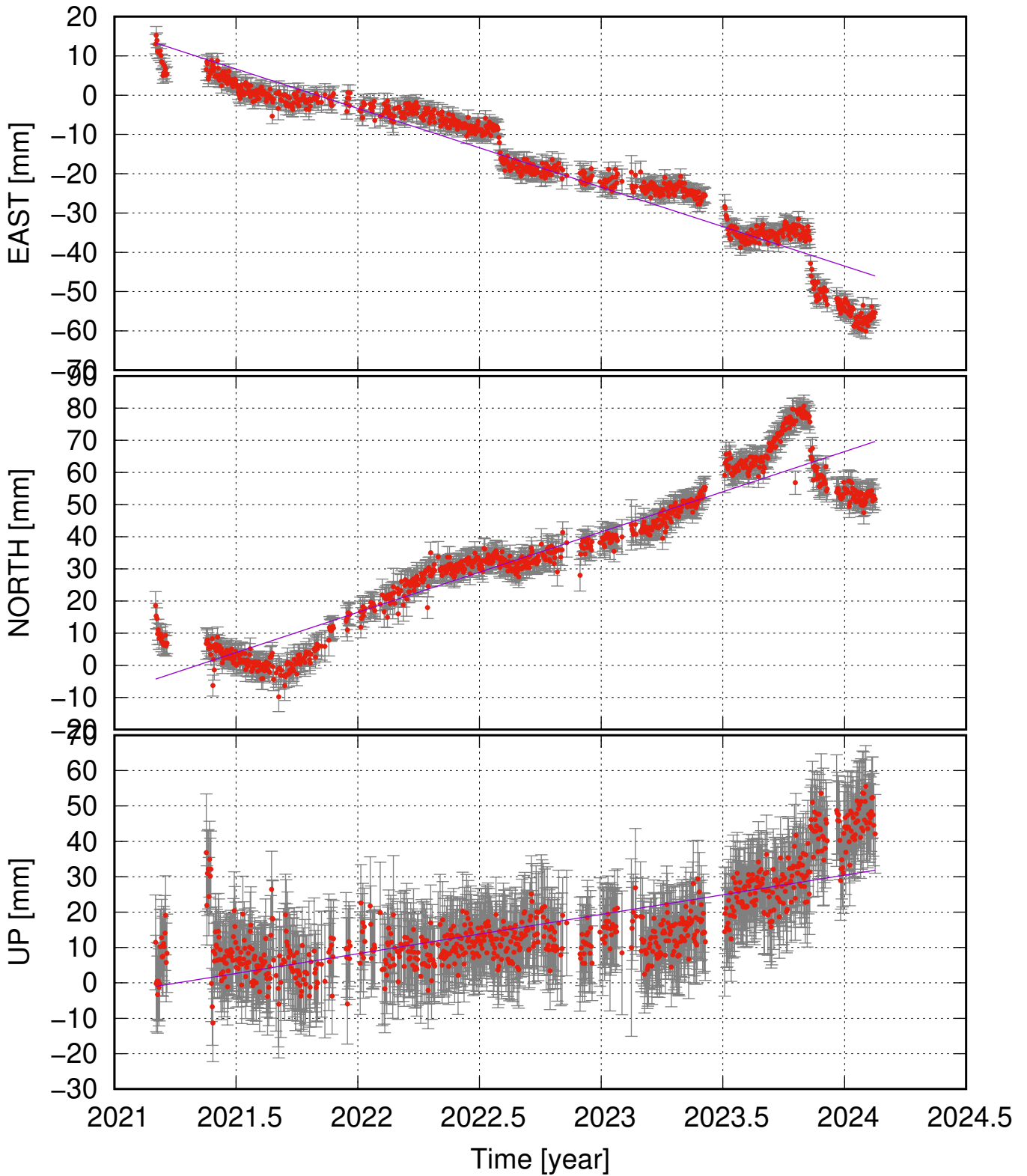
HVAS (64.02, -22.13) time series (ITRF 2014) v_e = -20.05 \pm 1.69 ; v_n = 25.00 \pm 2.50 ; v_u = 11.11 \pm 2.82 mm/yr
