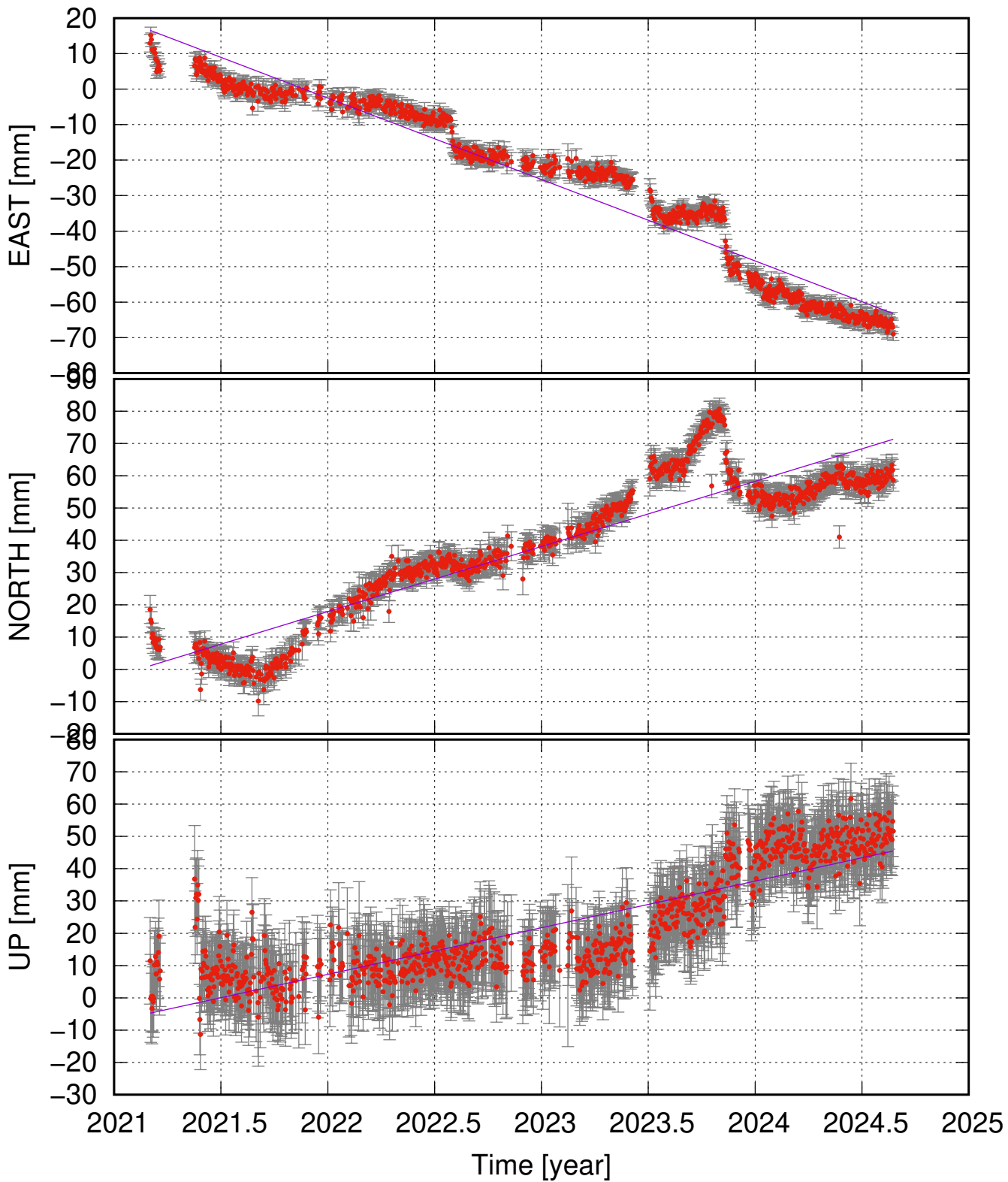
HVAS (64.02, -22.13) time series (ITRF 2014) v_e = -22.95 \pm 1.63 ; v_n = 20.19 \pm 2.54 ; v_u = 14.44 \pm 2.49 mm/yr
