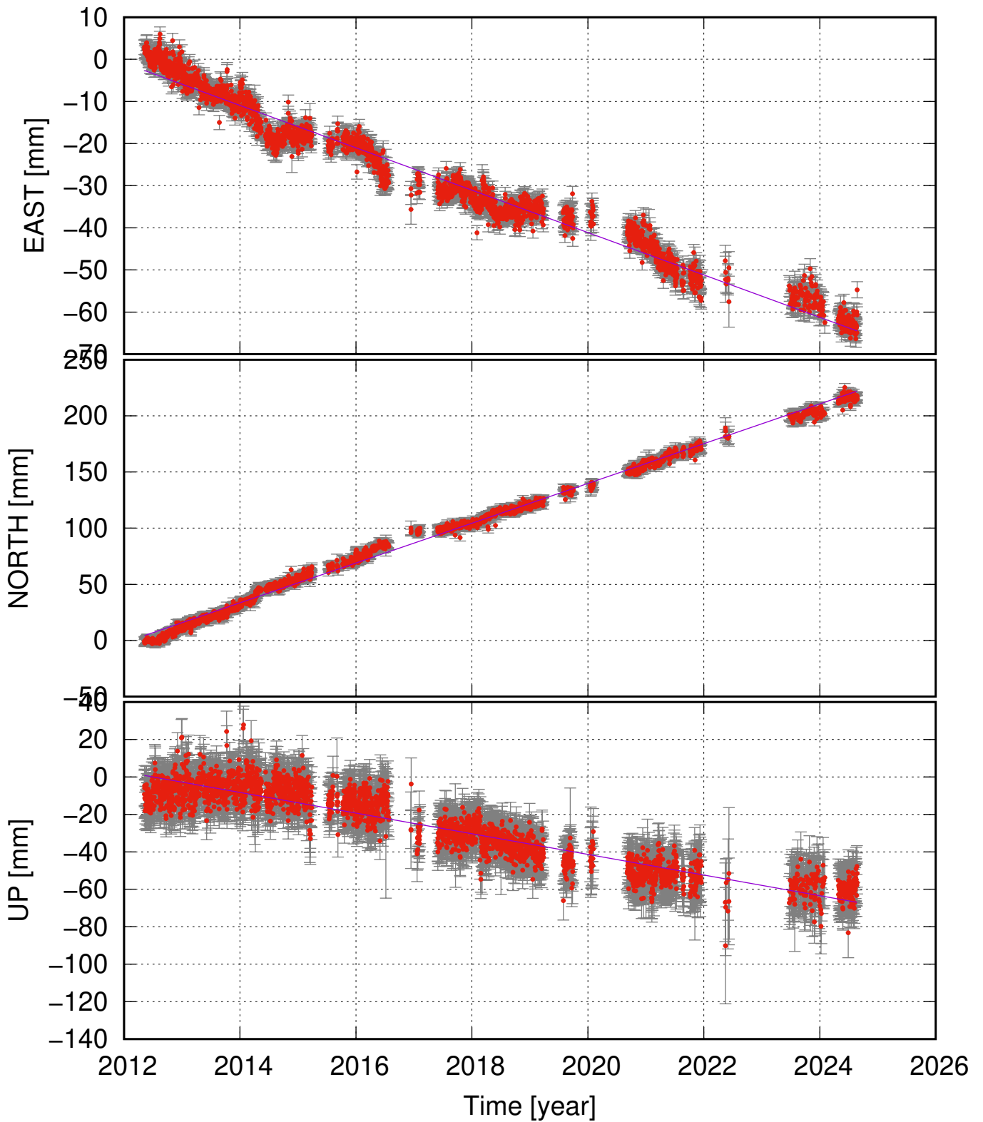
HUSM (64.07, -21.42) time series (ITRF 2014) v_e = -5.03 \pm 0.24 ; v_n = 17.70 \pm 0.35 ; v_u = -5.51 \pm 0.59 mm/yr
