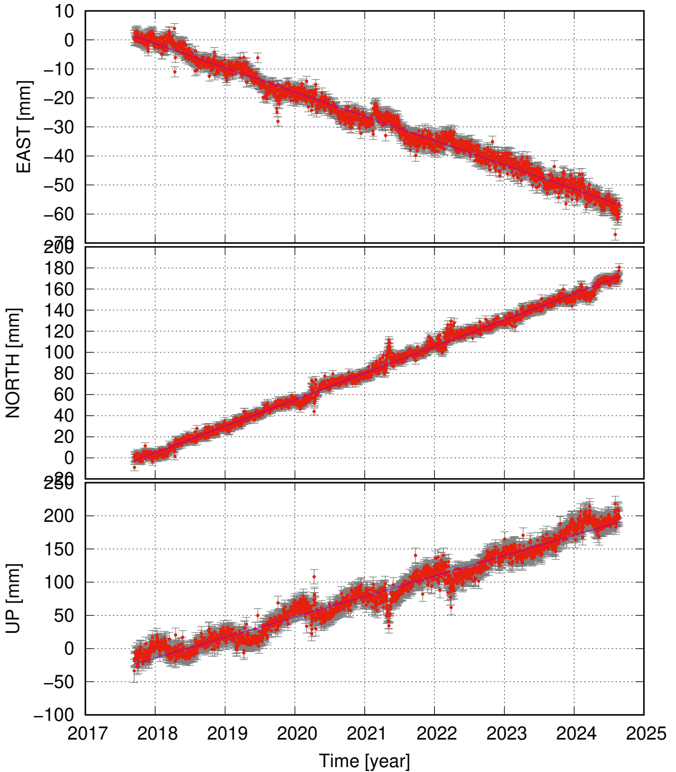
HSKC (64.62, -18.08) time series (ITRF 2014) v_e = -8.37 \pm 0.29 ; v_n = 25.14 \pm 0.50 ; v_u = 30.82 \pm 1.62 mm/yr
