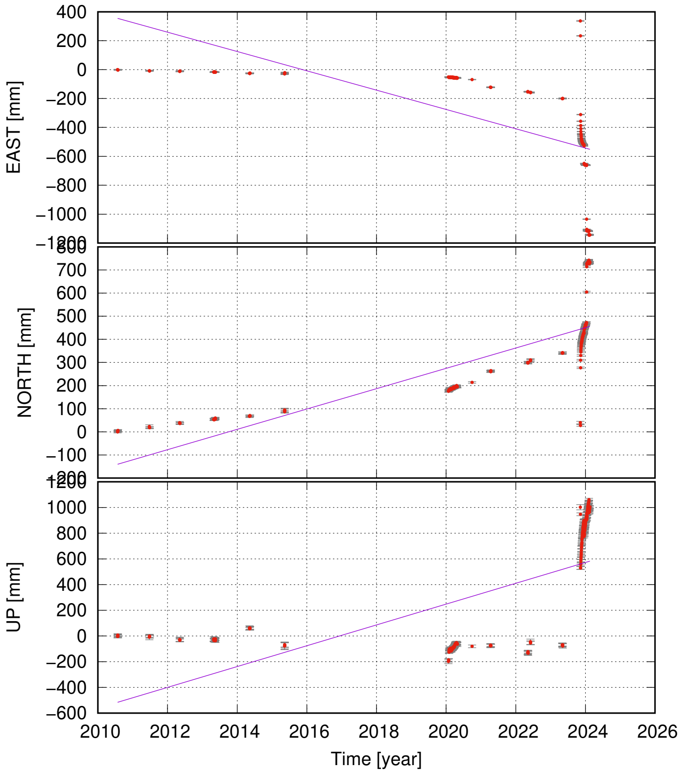
HS02 (63.87, -22.46) time series (ITRF 2014) v_e = -66.85 \pm 21.67 ; v_n = 43.95 \pm 9.69 ; v_u = 80.94 \pm 25.97 mm/yr
