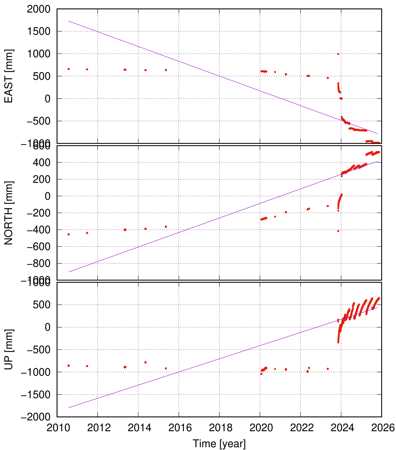
HS02 (, ) time series (IGb20) ve = +- ; vn = +- ; vu = +- mm/yr
