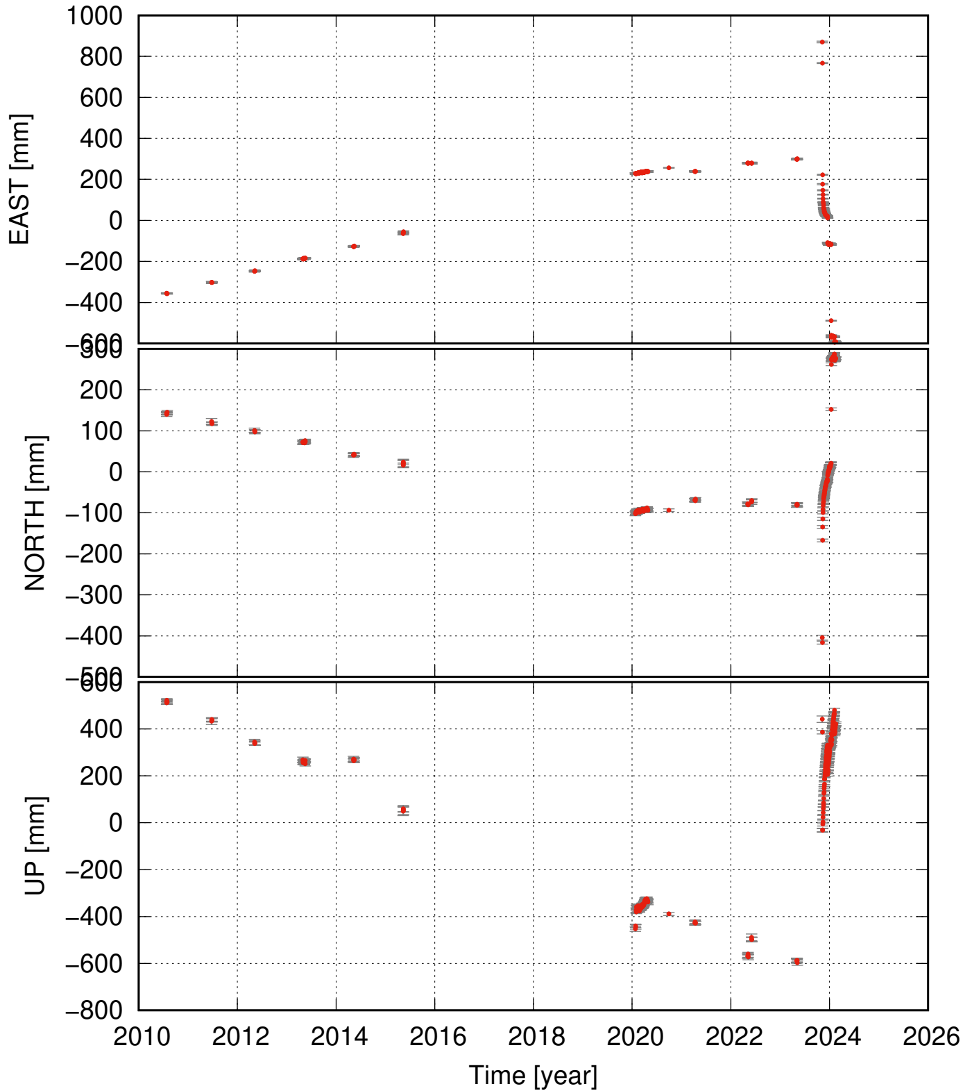
HS02 residual time series (some major events removed as well)
