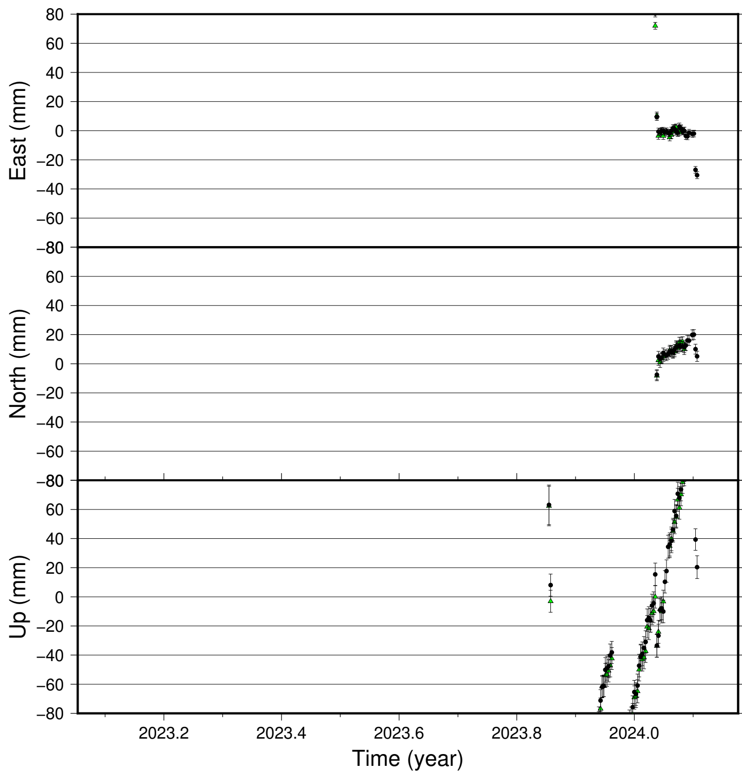
HS02 time series (IGS 2014), last 400 days
