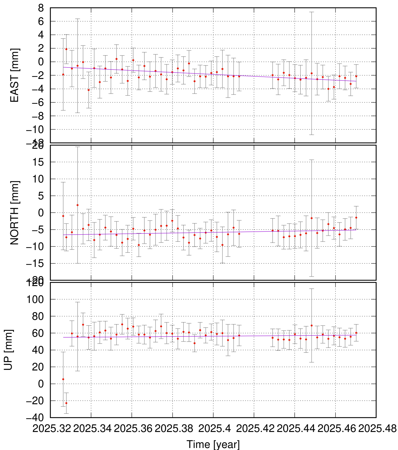
HRAH (64.90, -22.21) time series (ITRF 2020) ve = -14.41 ± 6.93; vn = 9.76 ± 16.08; vu = 18.47 ± 101.96 mm/yr
