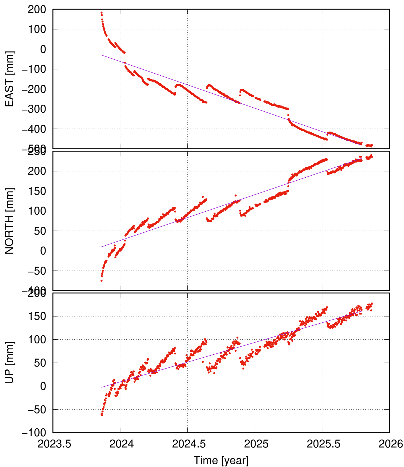
HRAG ( , ) time series (IGb20) ve = +- ; vn = +- ; vu = +- mm/yr
