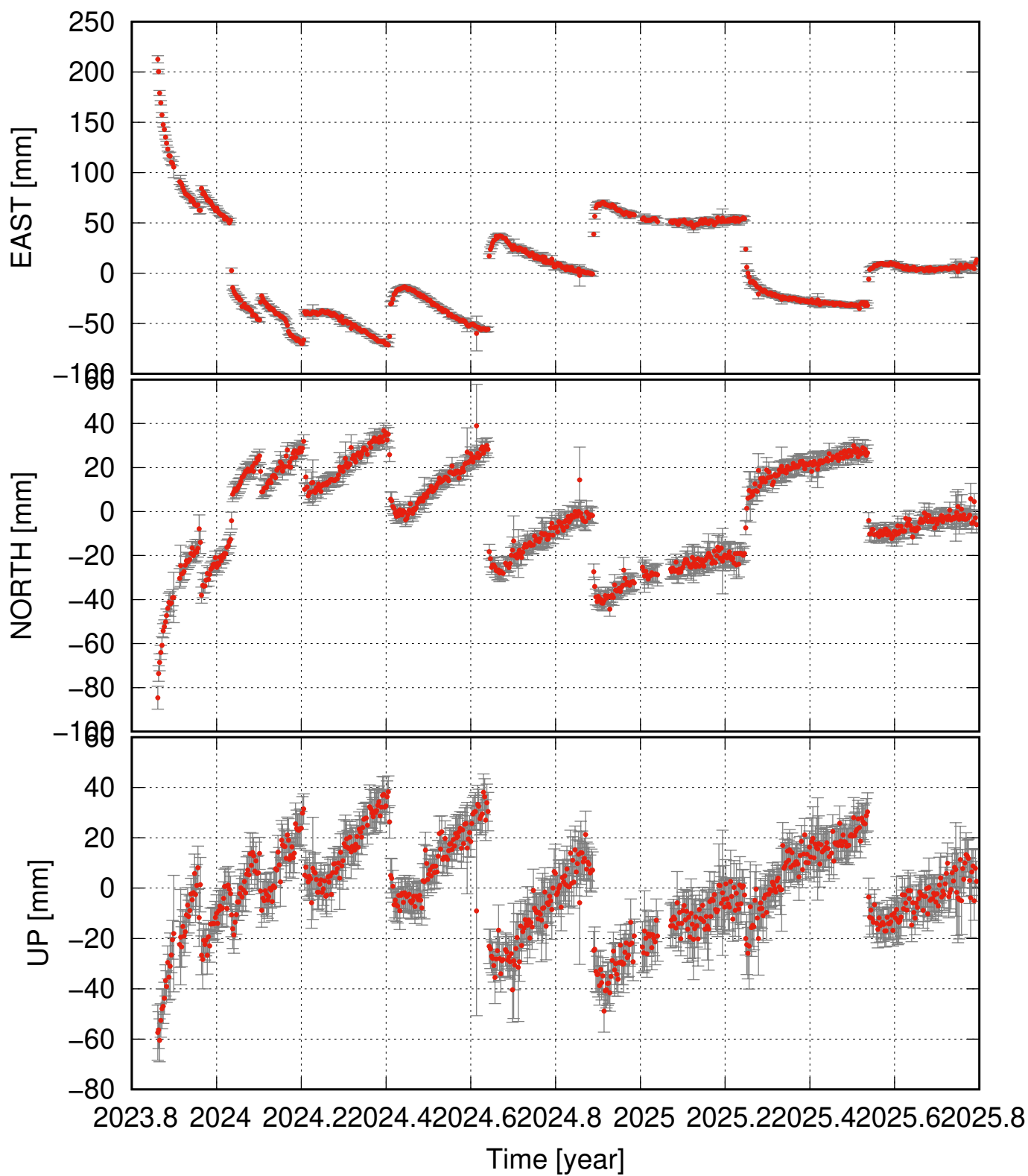
HRAG residual time series (some major events removed as well)
