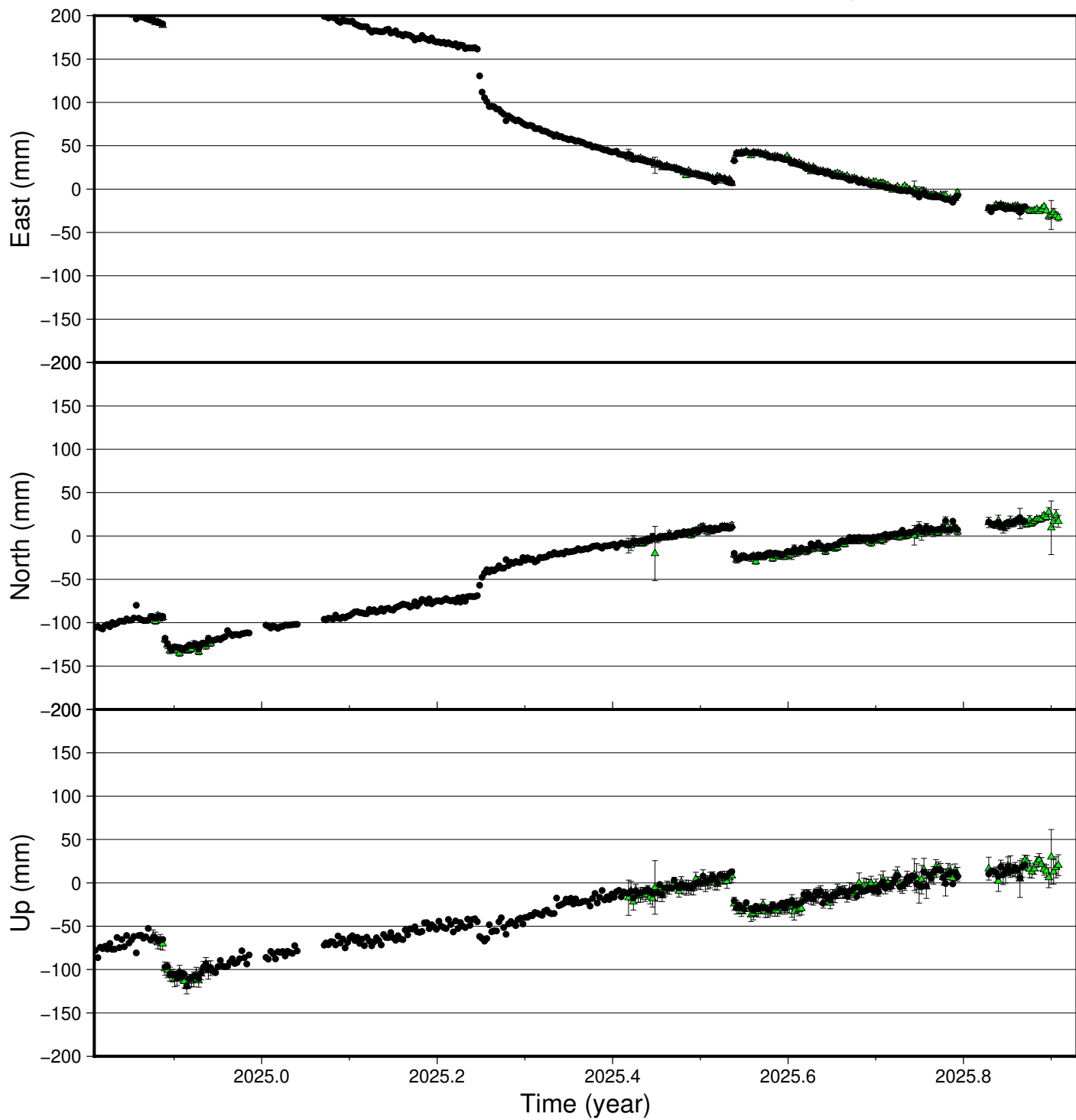
HRAG time series (ITRF2020), last 400 days
