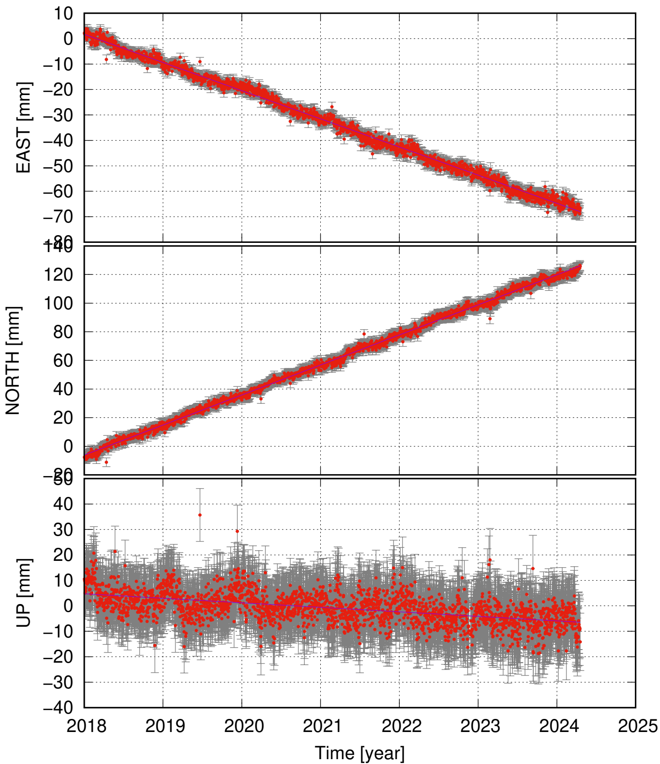
HRAC (66.11, -20.12) time series (ITRF 2014) v_e = -11.07 \pm 0.24 ; v_n = 20.98 \pm 0.29 ; v_u = -1.77 \pm 0.80 mm/yr
