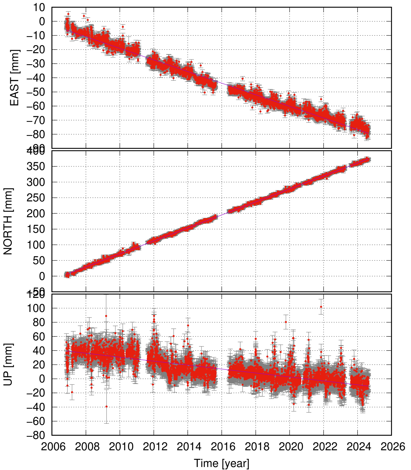
HOTJ (66.16, -17.24) time series (ITRF 2014) v_e = -4.11 \pm 0.15 ; v_n = 20.71 \pm 0.15 ; v_u = -2.80 \pm 0.59 mm/yr
