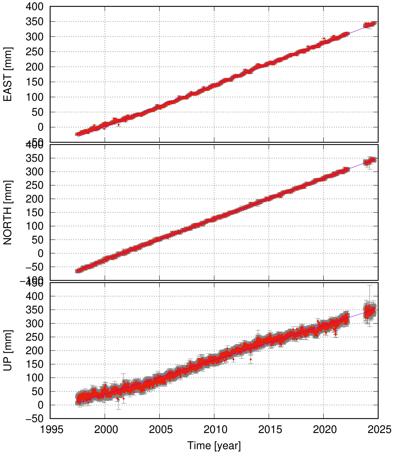
HOFN (64.27, -15.20) time series (ITRF 2014) v_e = 13.80 \pm 0.14 ; v_n = 15.00 \pm 0.09 ; v_u = 12.64 \pm 0.34 mm/yr
