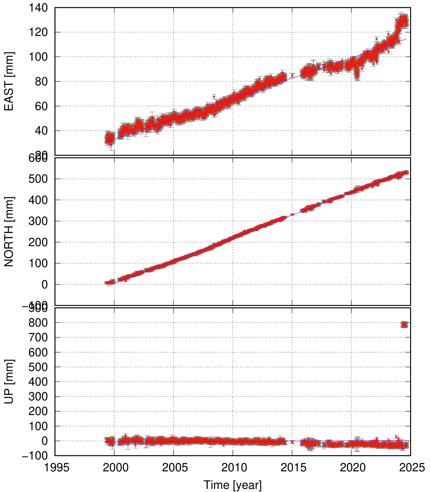
HLID (63.92, -21.39) time series (ITRF 2014) v_e = 3.30 \pm 0.17 ; v_n = 21.56 \pm 0.18 ; v_u = 0.46 \pm 3.22 mm/yr
