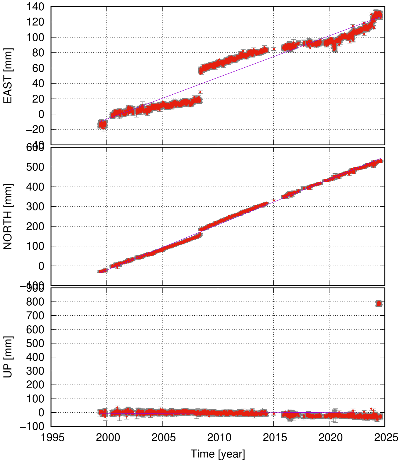
HLID (63.92, -21.39) time series (ITRF 2014) v_e = 5.42 \pm 0.48 ; v_n = 22.93 \pm 0.39 ; v_u = 0.46 \pm 3.22 mm/yr
