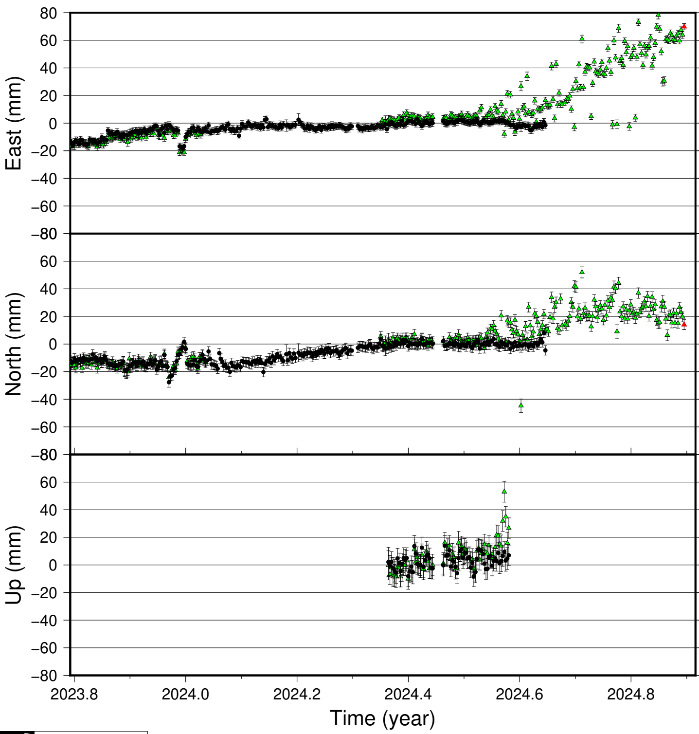
HLID time series (IGS 2014), last 400 days
