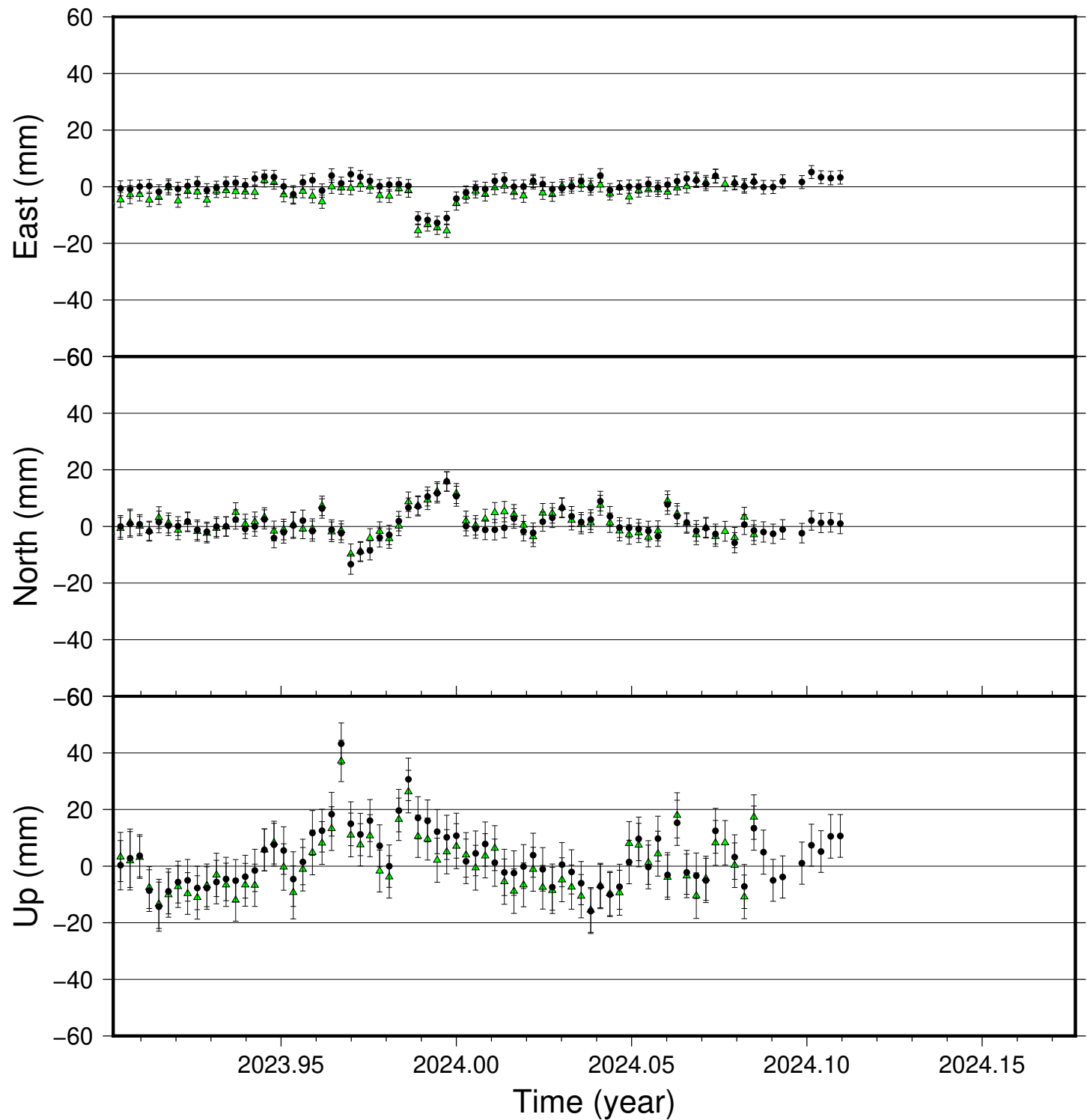
HLID time series (IGS 2014), last 100 days
