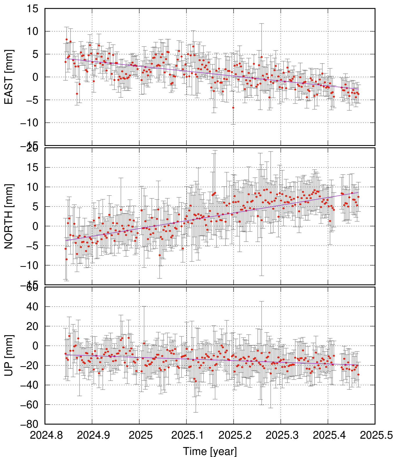
HITA (64.80, -22.04) time series (IGb20) v_e = -10.77 \pm 3.24 ; v_n = 19.82 \pm 3.74 ; v_u = -16.65 \pm 11.28 mm/yr
