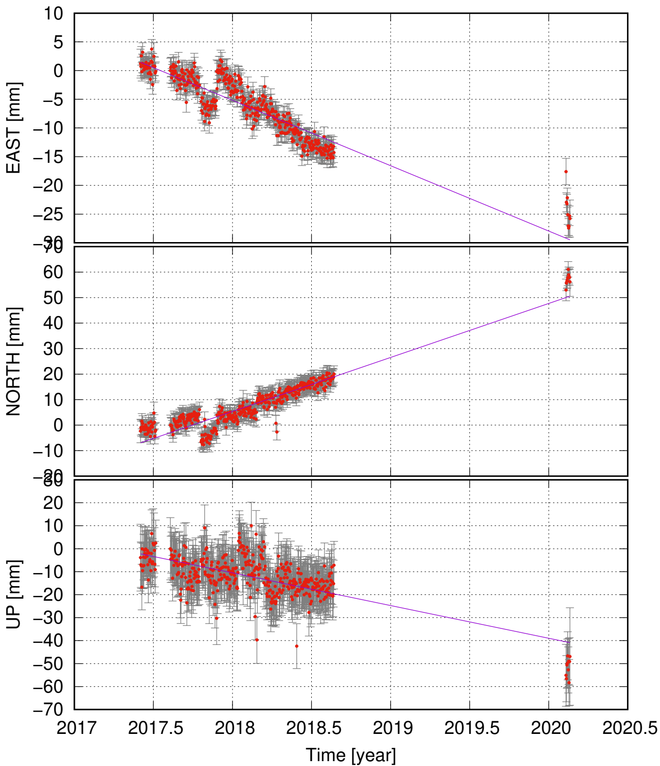
HESS (64.03, -21.37) time series (ITRF 2014) v_e = -11.39 \pm 0.85 ; v_n = 21.16 \pm 1.28 ; v_u = -14.23 \pm 2.43 mm/yr
