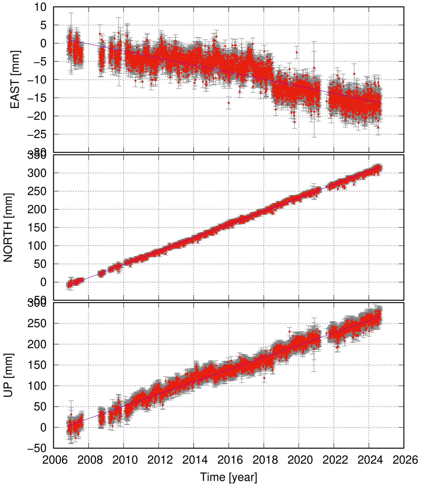
HESA (64.05, -19.56) time series (ITRF 2014) v_e = -0.97 \pm 0.14 ; v_n = 18.32 \pm 0.18 ; v_u = 14.70 \pm 0.51 mm/yr
