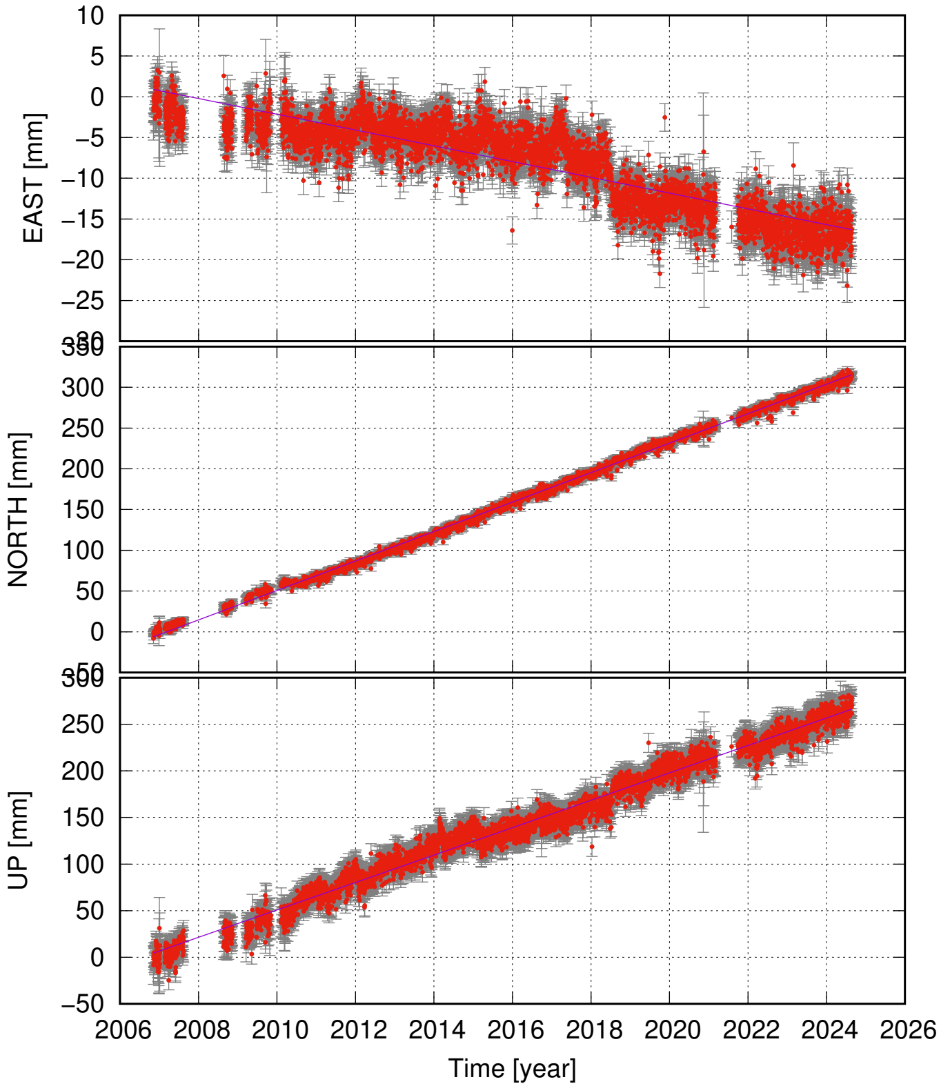
HESA (64.05, -19.56) time series (ITRF 2014) v_e = -0.97 \pm 0.14 ; v_n = 18.08 \pm 0.21 ; v_u = 14.70 \pm 0.51 mm/yr
