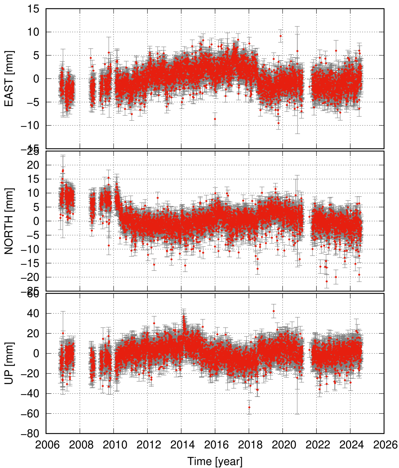
HESA detrended and seasonal signal removed
