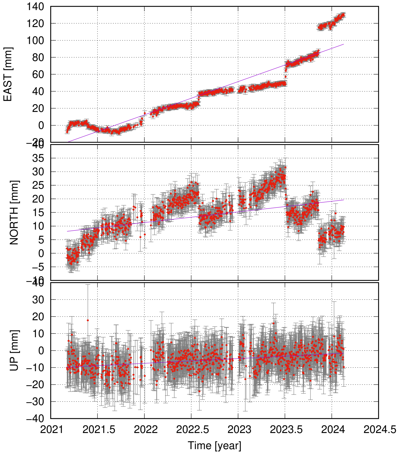
HERV (63.87, -21.88) time series (ITRF 2014) v_e = 39.11 \pm 4.57 ; v_n = 3.92 \pm 2.22 ; v_u = 2.79 \pm 1.84 mm/yr
