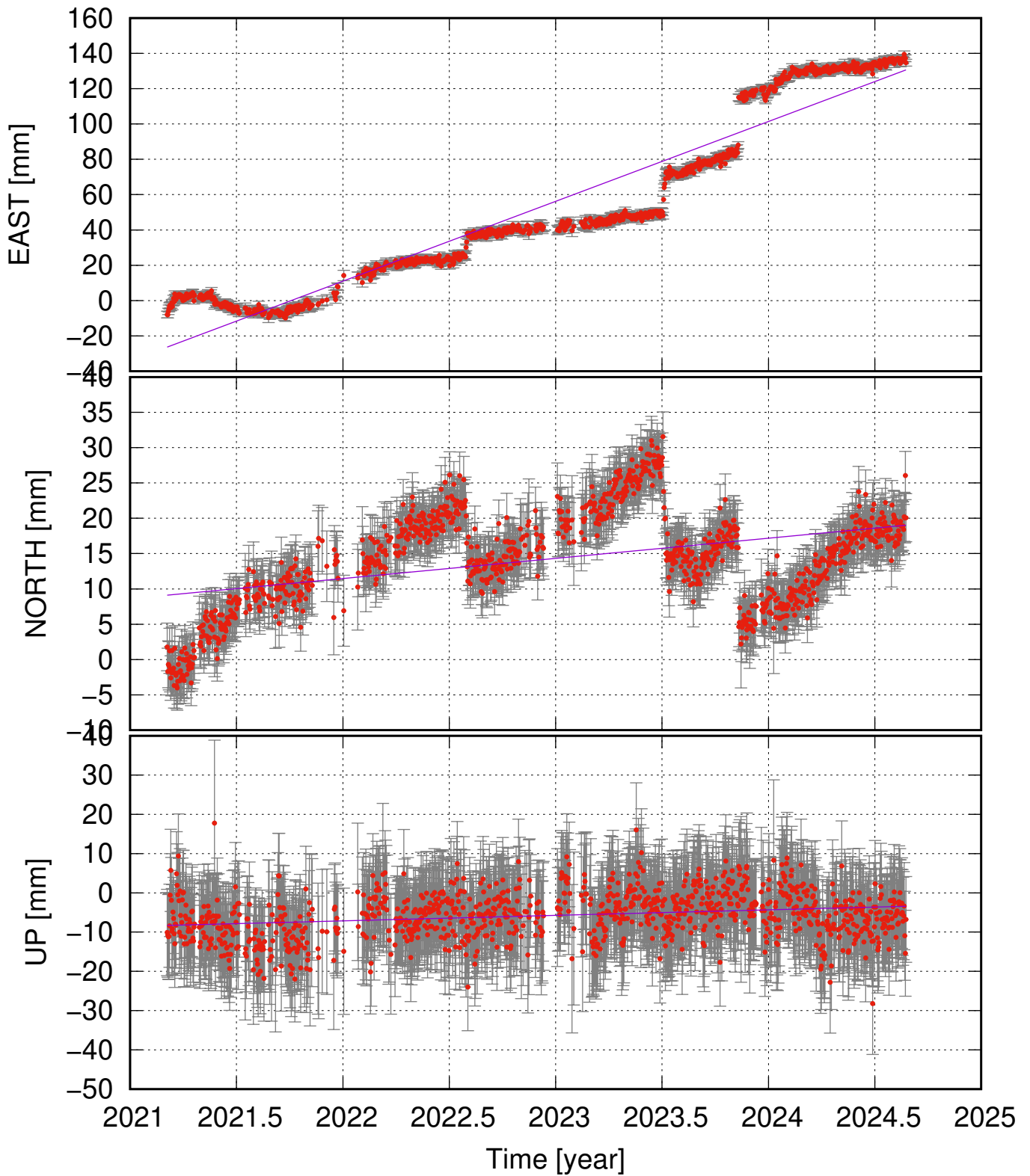
HERV (63.87, -21.88) time series (ITRF 2014) v_e = 45.20 \pm 4.22 ; v_n = 2.85 \pm 1.81 ; v_u = 1.41 \pm 1.63 mm/yr
