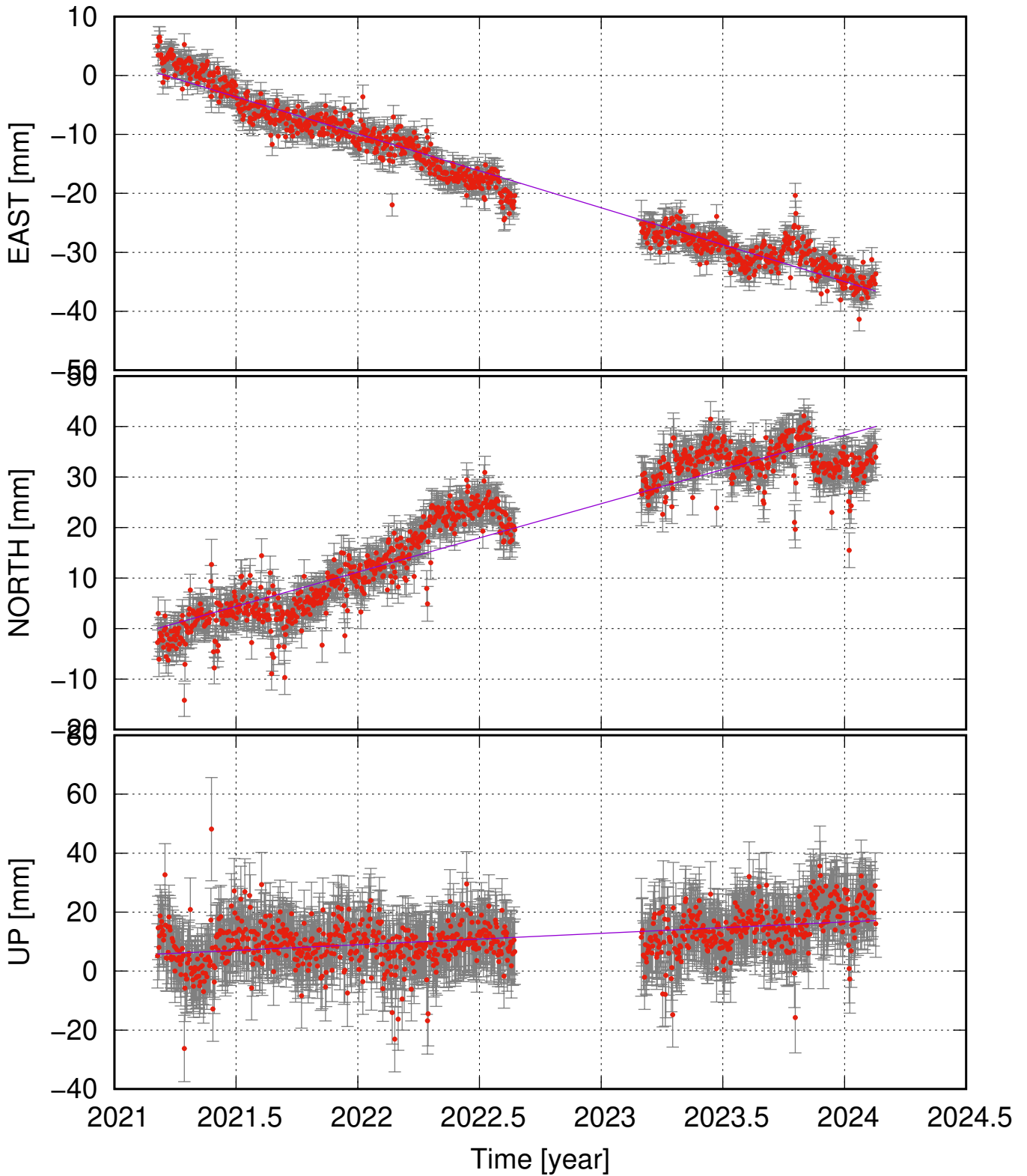
HELF (64.02, -21.85) time series (ITRF 2014) v_e = -12.53 \pm 0.76 ; v_n = 13.54 \pm 1.57 ; v_u = 3.86 \pm 2.40 mm/yr
