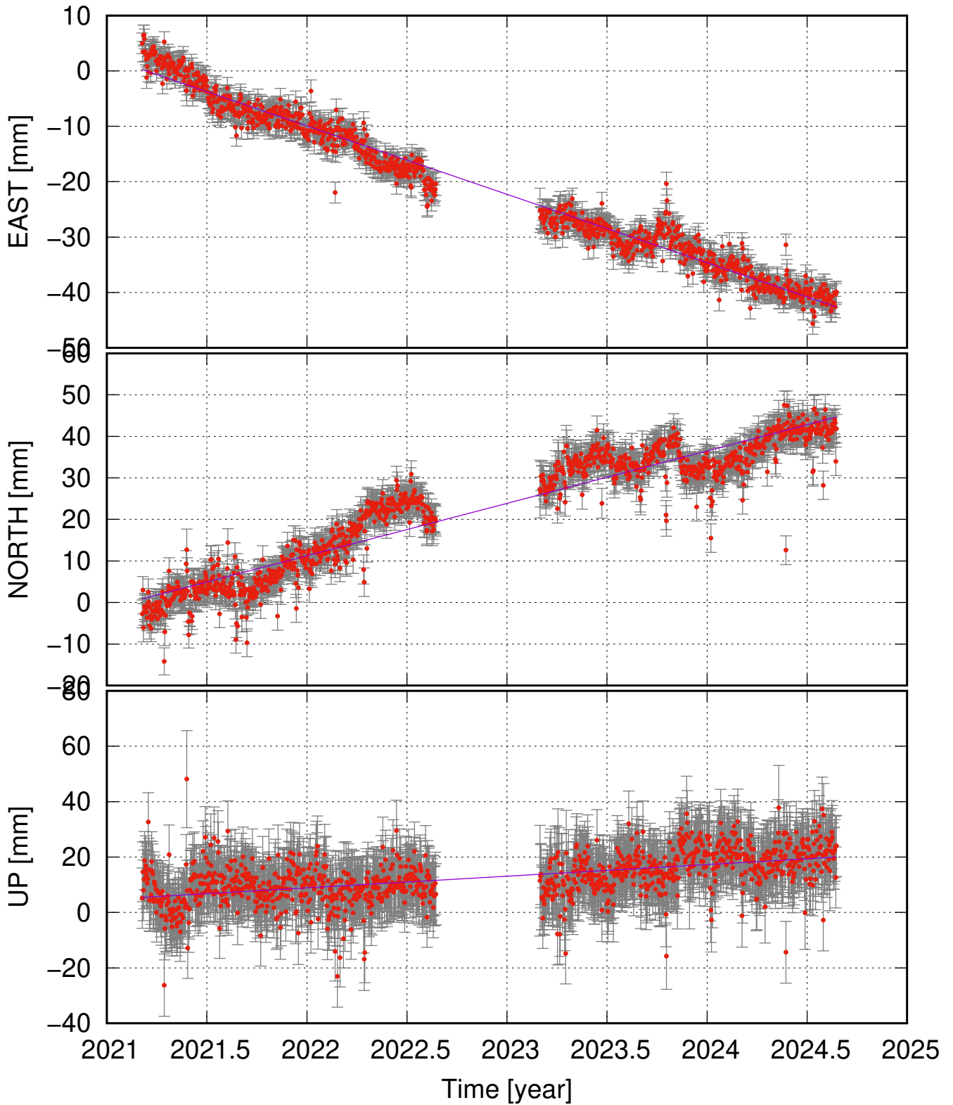
HELF (64.02, -21.85) time series (ITRF 2014) v_e = -12.36 \pm 0.62 ; v_n = 12.63 \pm 1.34 ; v_u = 4.19 \pm 2.03 mm/yr
