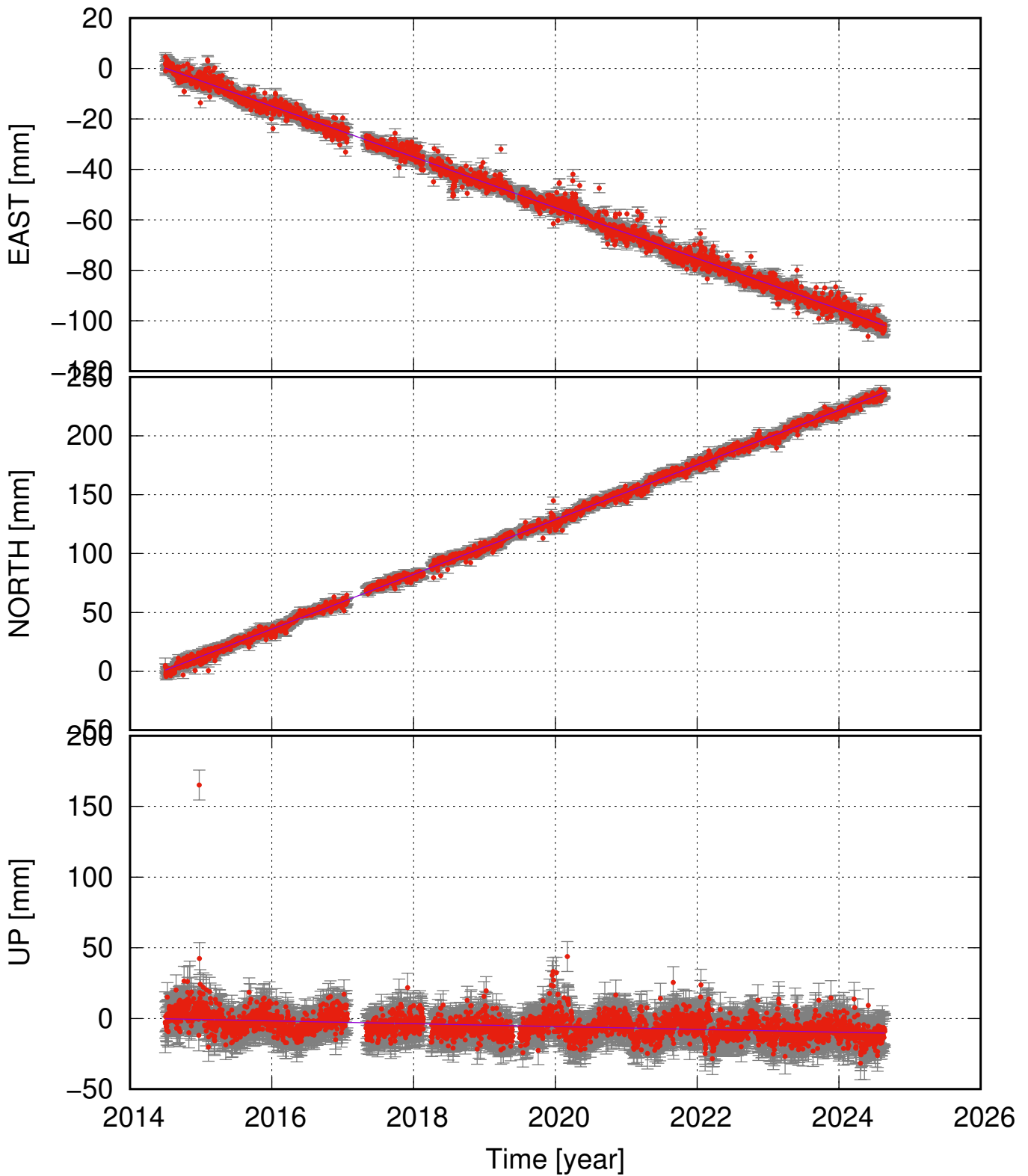
HELC (65.94, -18.39) time series (ITRF 2014) v_e = -10.06 \pm 0.20 ; v_n = 23.23 \pm 0.23 ; v_u = -1.01 \pm 0.73 mm/yr
