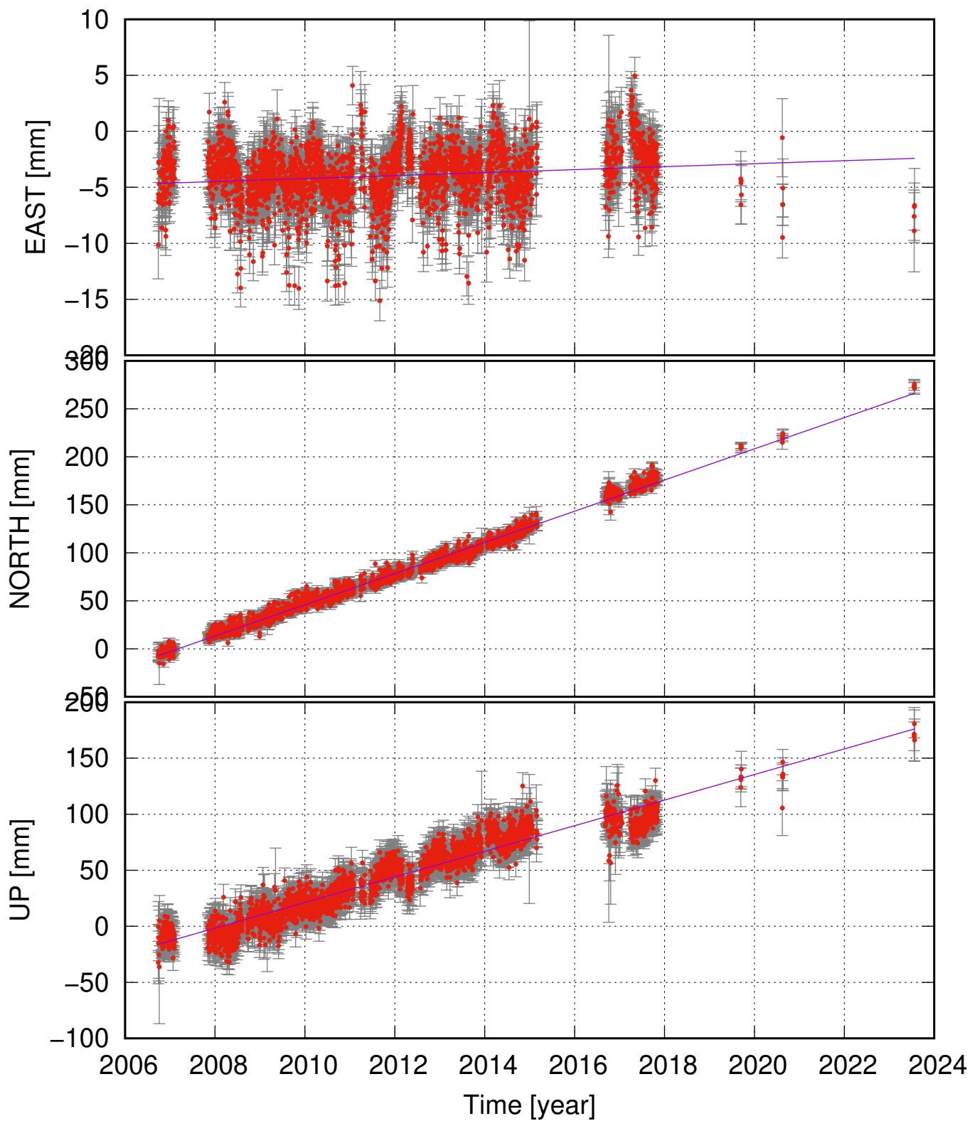
HEKR (64.01, -19.66) time series (ITRF 2014) v_e = 0.13 \pm 0.14 ; v_n = 16.25 \pm 0.28 ; v_u = 11.43 \pm 0.64 mm/yr
