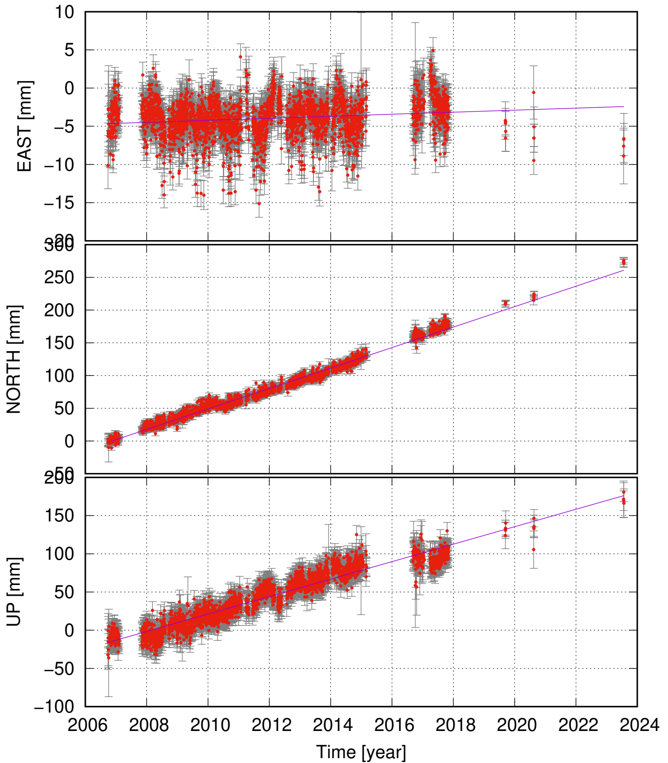
HEKR (64.01, -19.66) time series (ITRF 2014) v_e = 0.13 \pm 0.14 ; v_n = 15.62 \pm 0.32 ; v_u = 11.43 \pm 0.64 mm/yr
