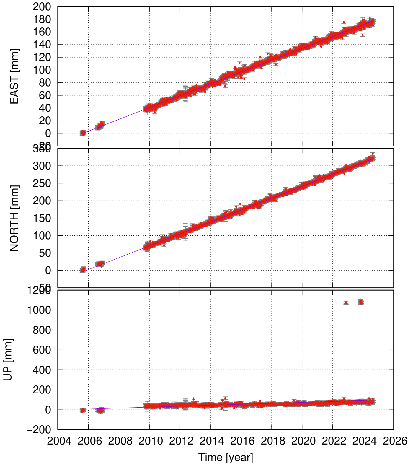
HEID (65.38, -14.54) time series (ITRF 2014) v_e = 9.33 \pm 0.12 ; v_n = 17.04 \pm 0.14 ; v_u = 4.71 \pm 4.10 mm/yr
