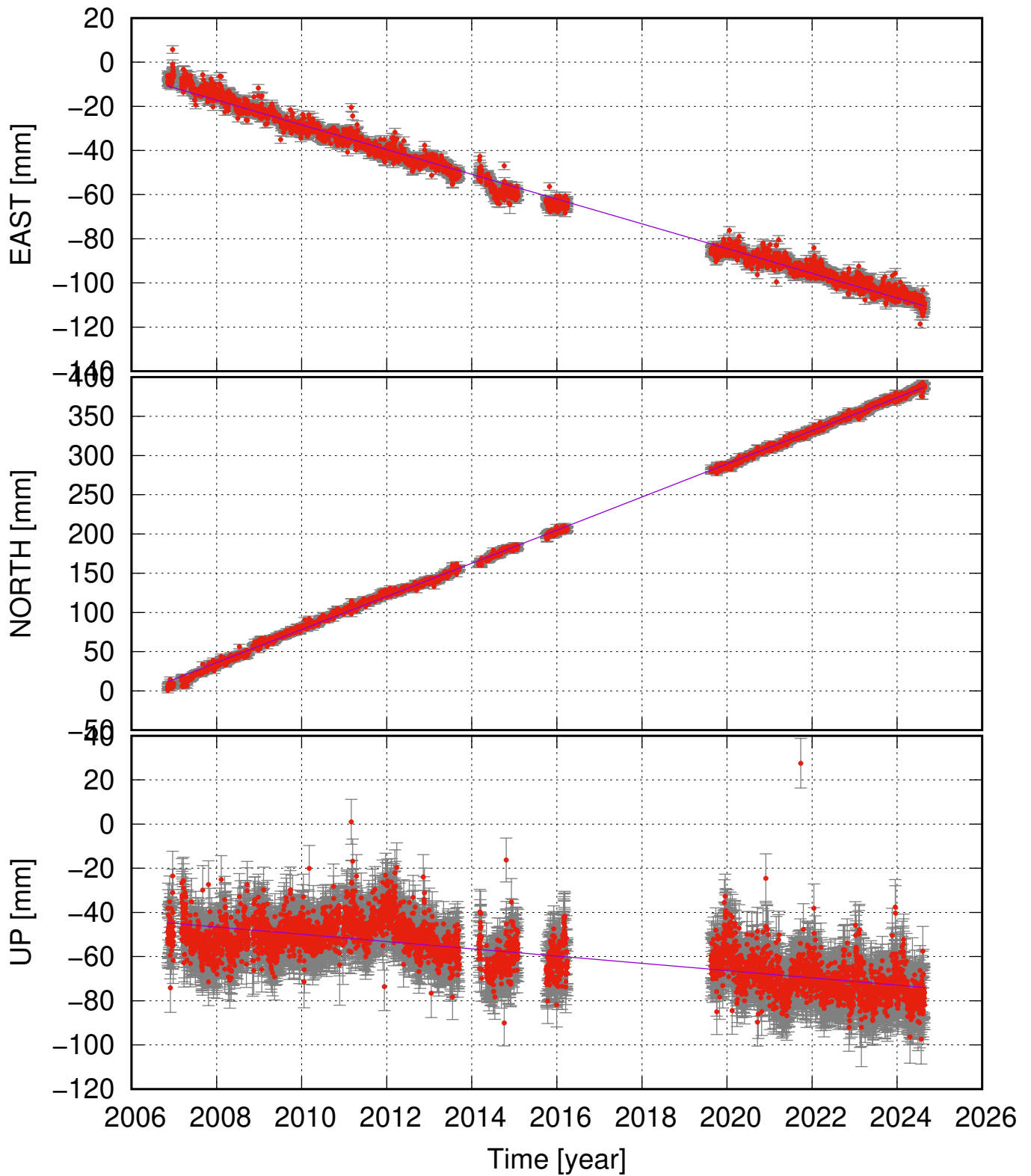
HEDI (66.08, -17.31) time series (ITRF 2014) v_e = -5.60 \pm 0.14 ; v_n = 21.10 \pm 0.16 ; v_u = -1.64 \pm 0.46 mm/yr
