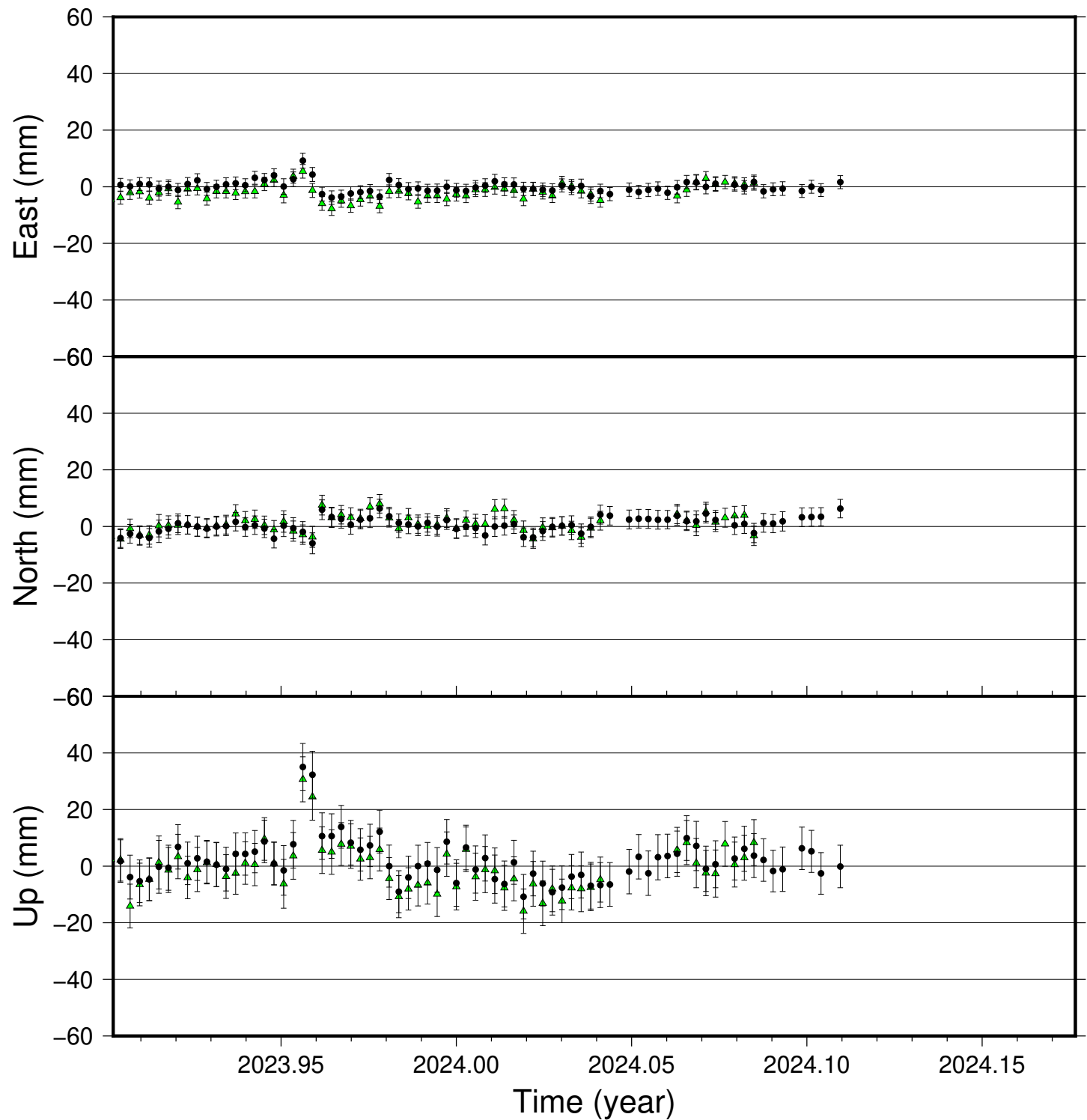
HEDI time series (IGS 2014), last 100 days
