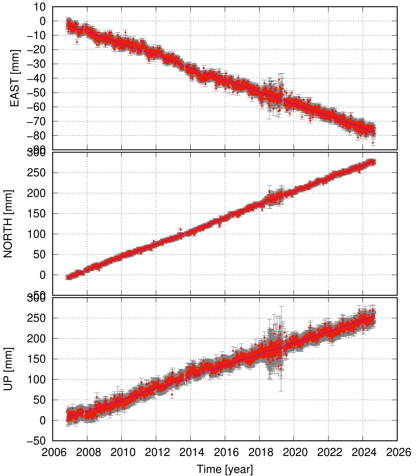
HAUD (63.97, -19.96) time series (ITRF 2014) v_e = -4.21 \pm 0.11 ; v_n = 16.02 \pm 0.15 ; v_u = 13.93 \pm 0.44 mm/yr
