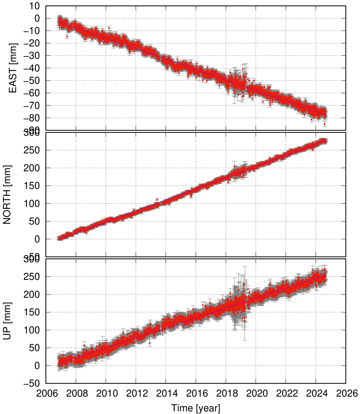
HAUD (63.97, -19.96) time series (ITRF 2014) v_e = -4.21 \pm 0.11 ; v_n = 15.64 \pm 0.20 ; v_u = 13.93 \pm 0.44 mm/yr
