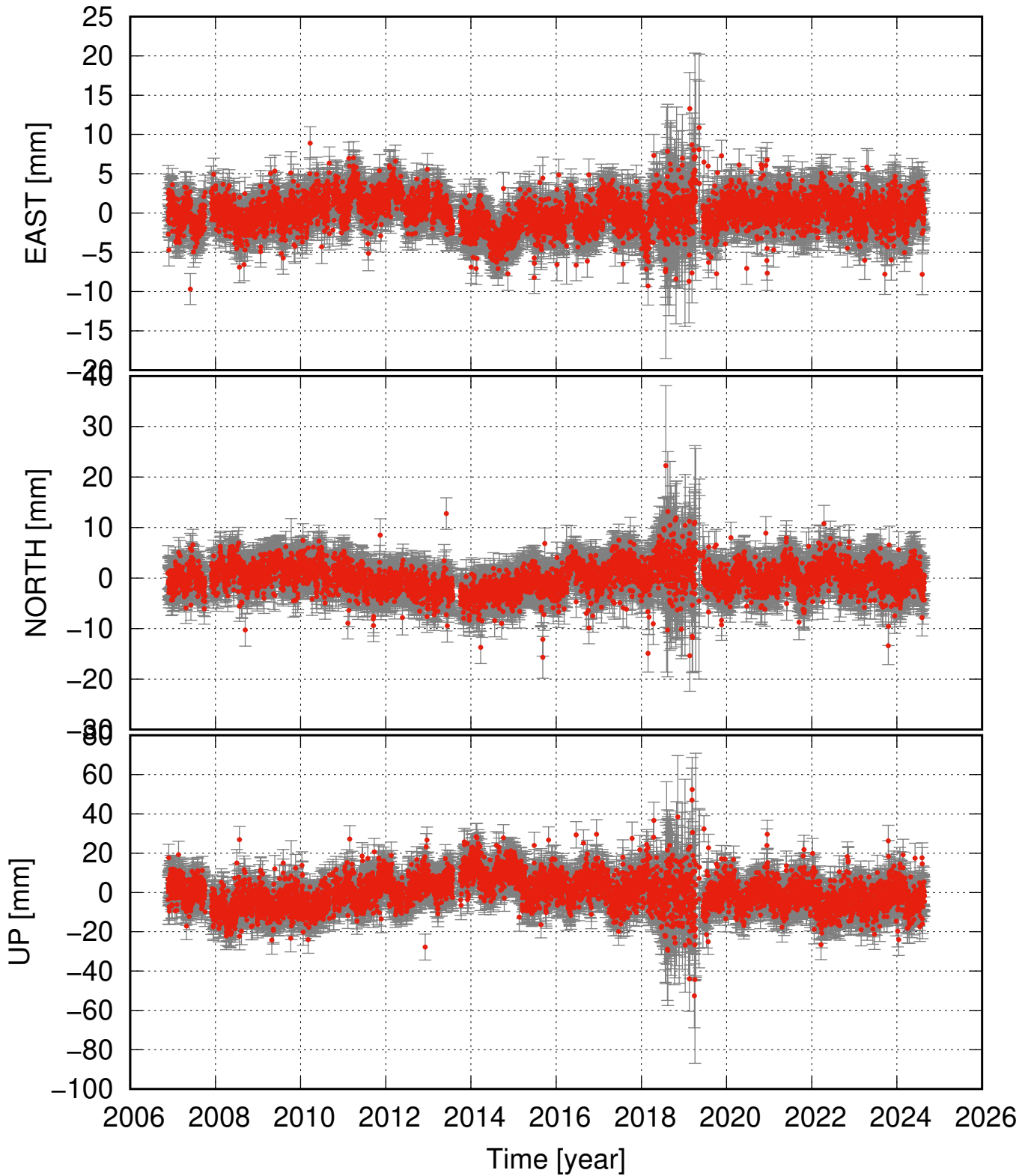
HAUD residual time series (some major events removed as well)
