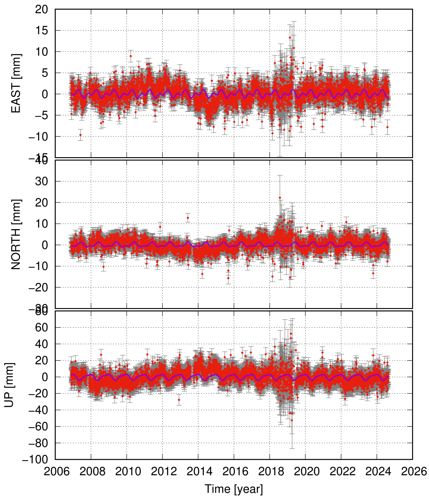
HAUD seasonal fit
