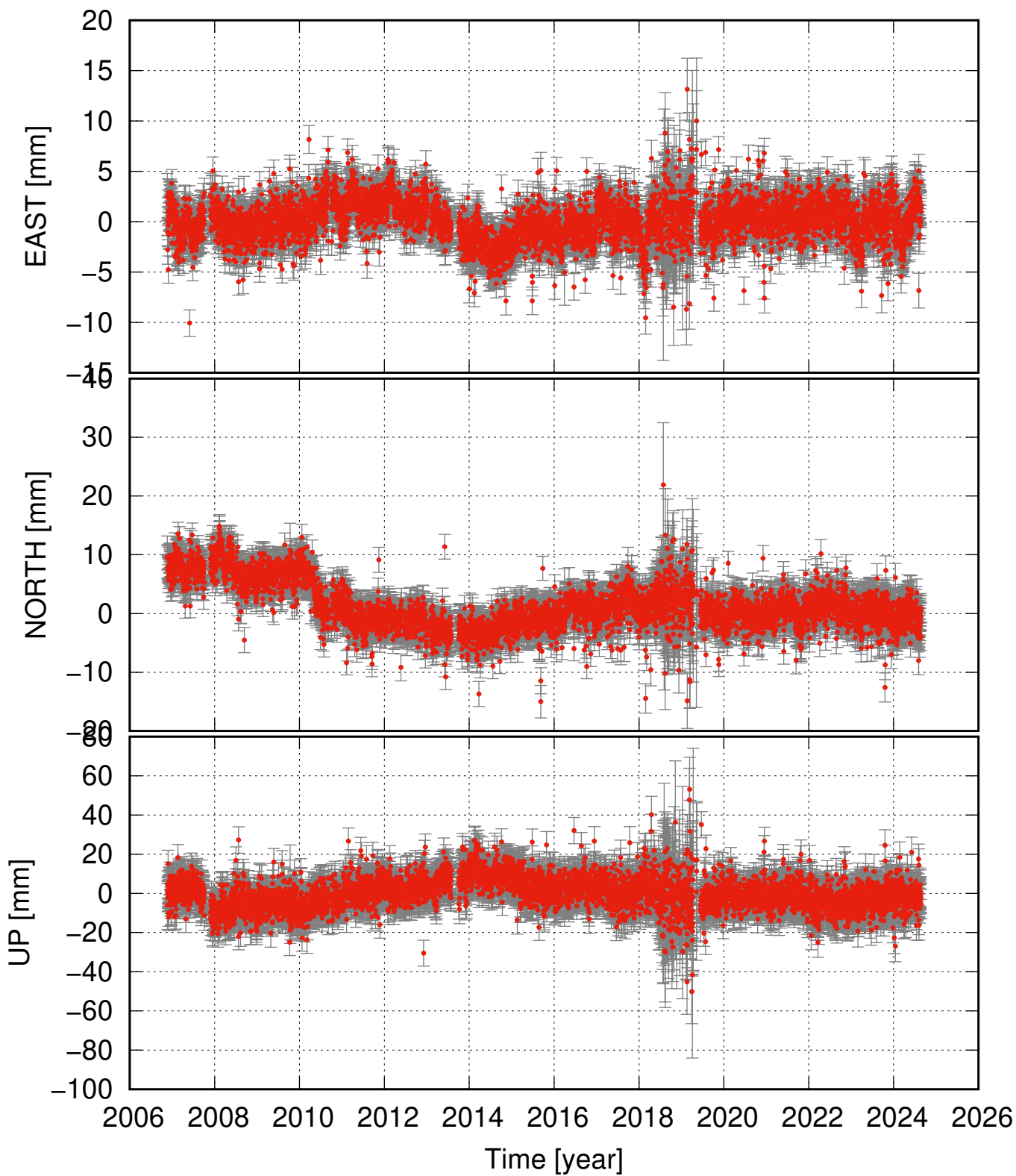
HAUD detrended and seasonal signal removed
