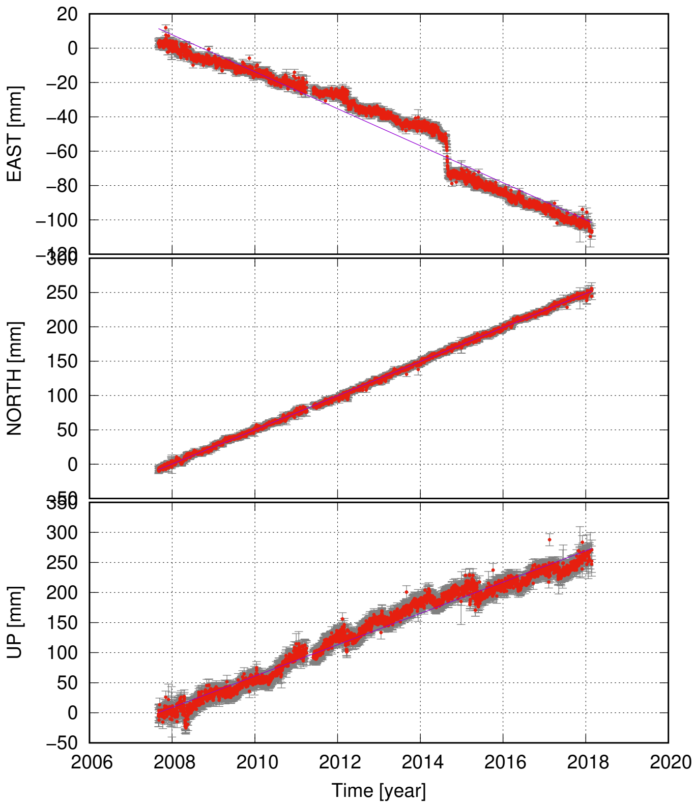
HAUC (64.71, -18.34) time series (ITRF 2014) v_e = -10.77 \pm 0.63 ; v_n = 24.81 \pm 0.20 ; v_u = 26.04 \pm 1.15 mm/yr
