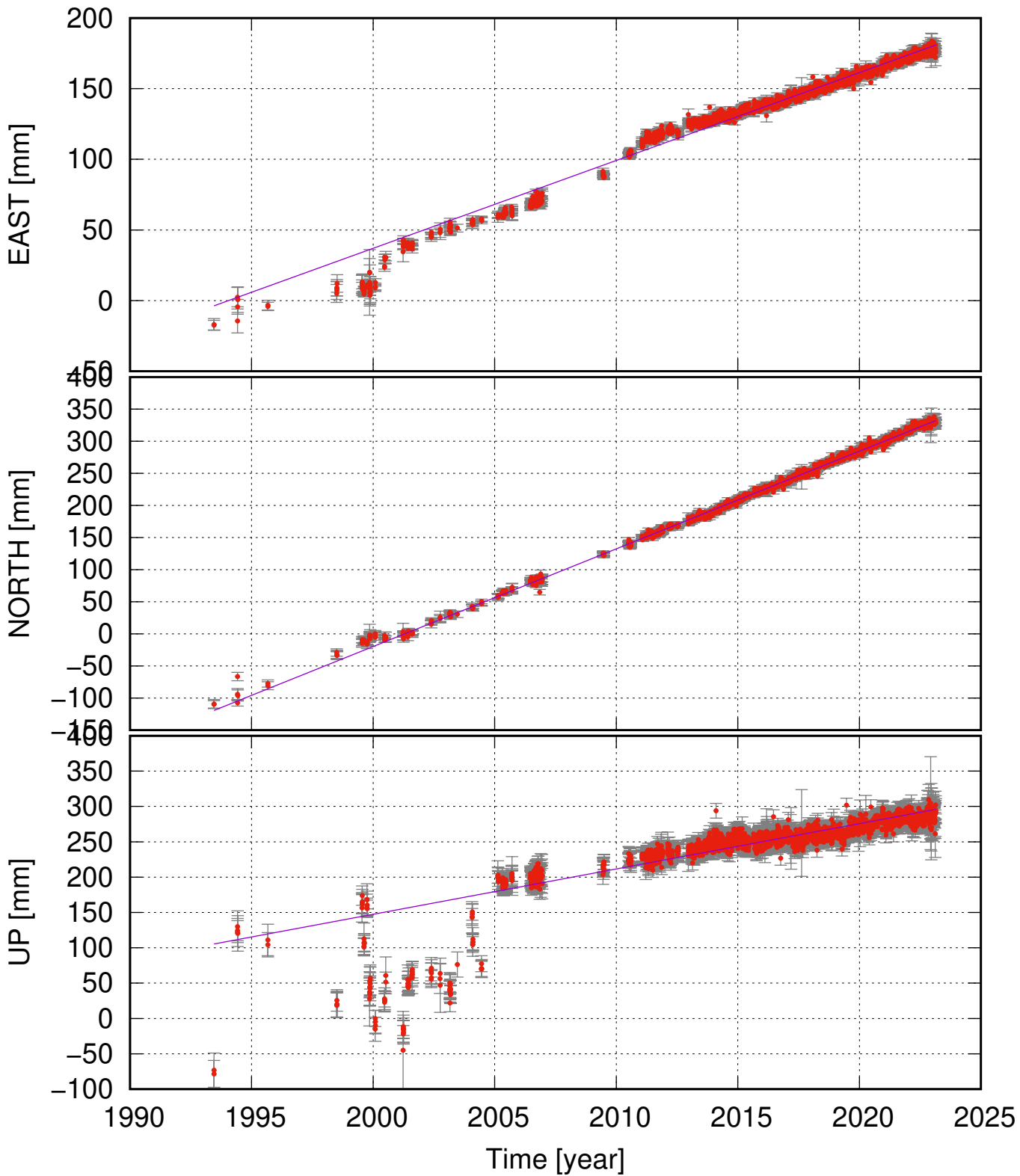
HAMR (63.62, -19.99) time series (ITRF 2014) v_e = 6.22 \pm 0.16 ; v_n = 15.21 \pm 0.10 ; v_u = 6.41 \pm 0.68 mm/yr
