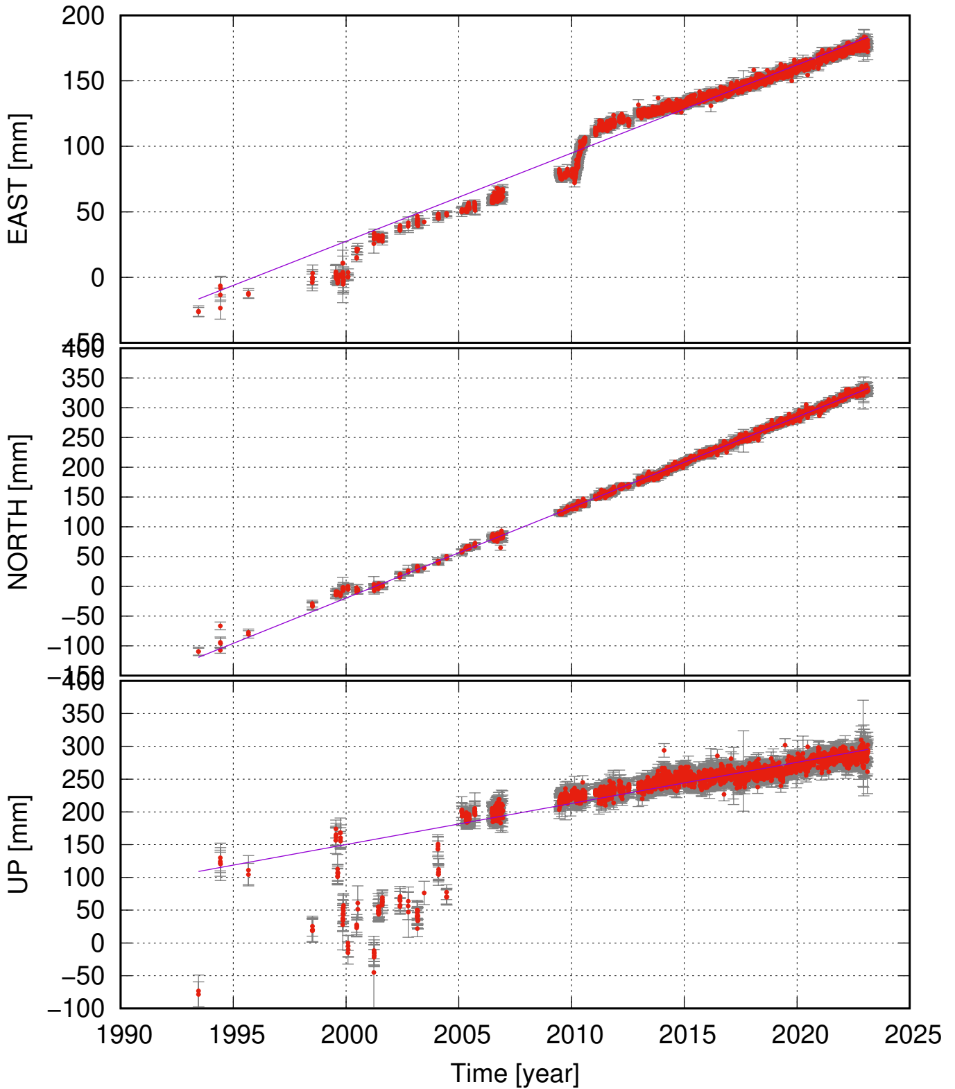
HAMR (63.62, -19.99) time series (ITRF 2014) v_e = 6.73 \pm 0.22 ; v_n = 15.21 \pm 0.10 ; v_u = 6.27 \pm 0.67 mm/yr
