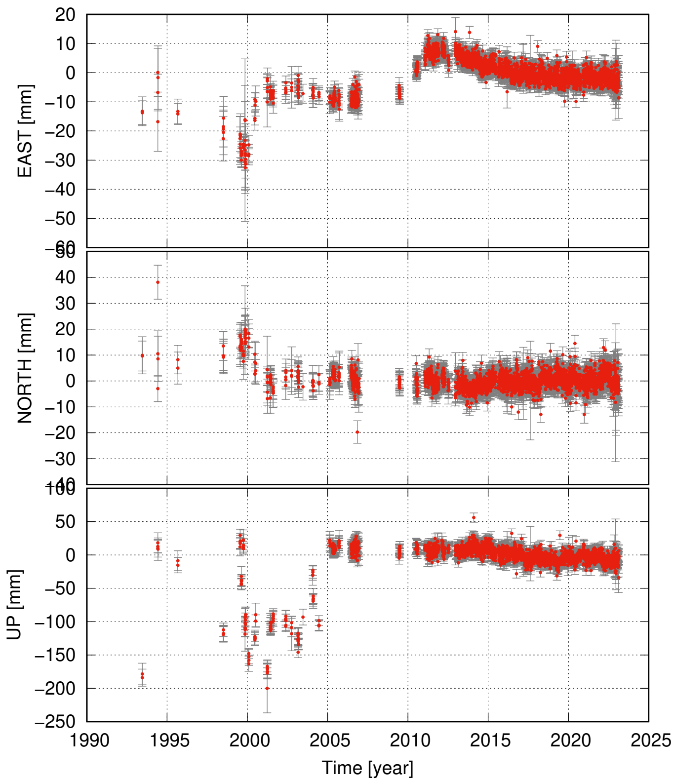
HAMR residual time series (some major events removed as well)
