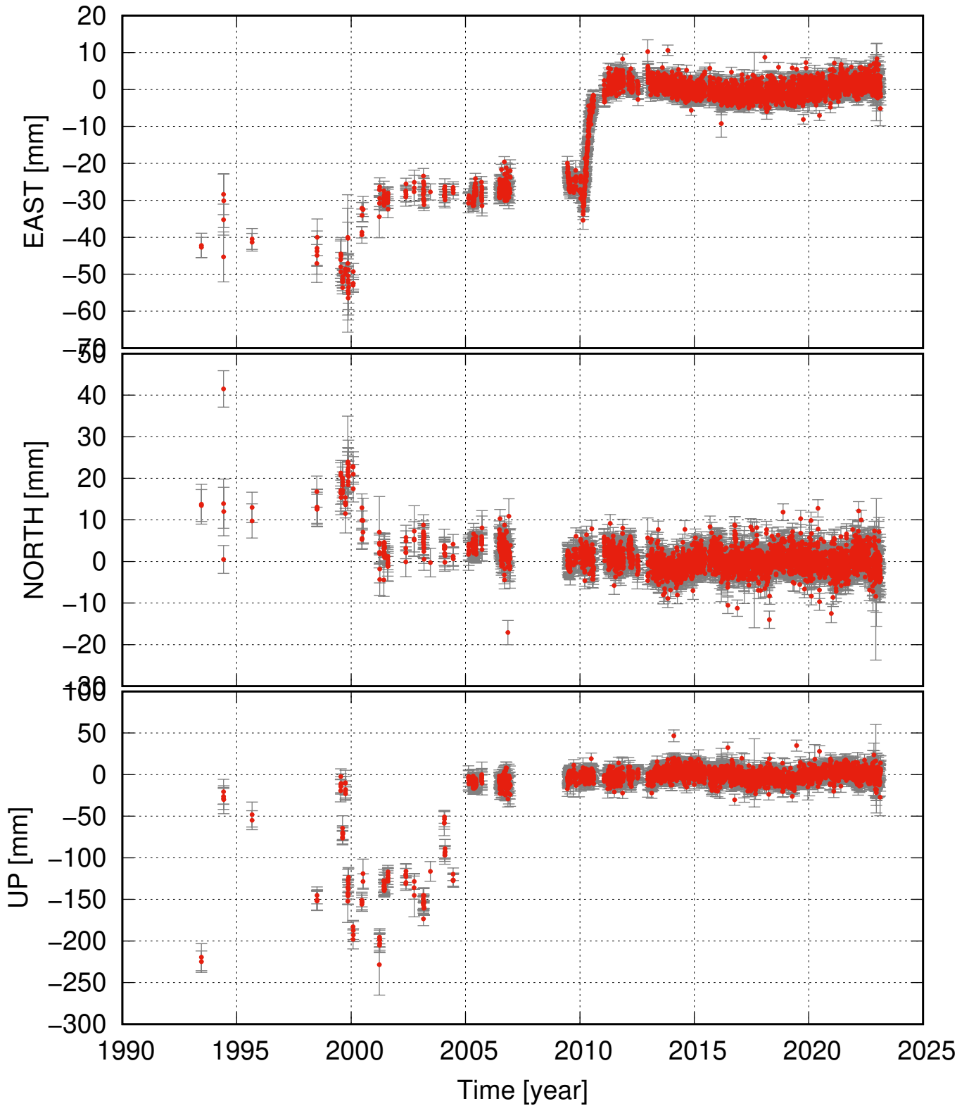
HAMR detrended and seasonal signal removed
